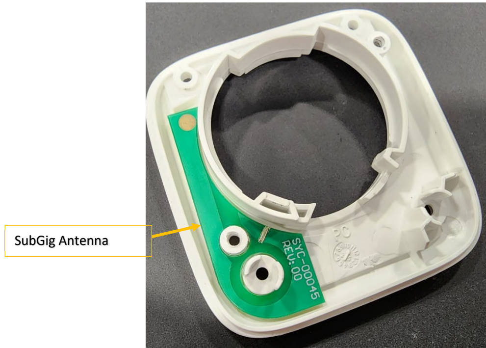
Figure 7 – PCB Antenna Front
