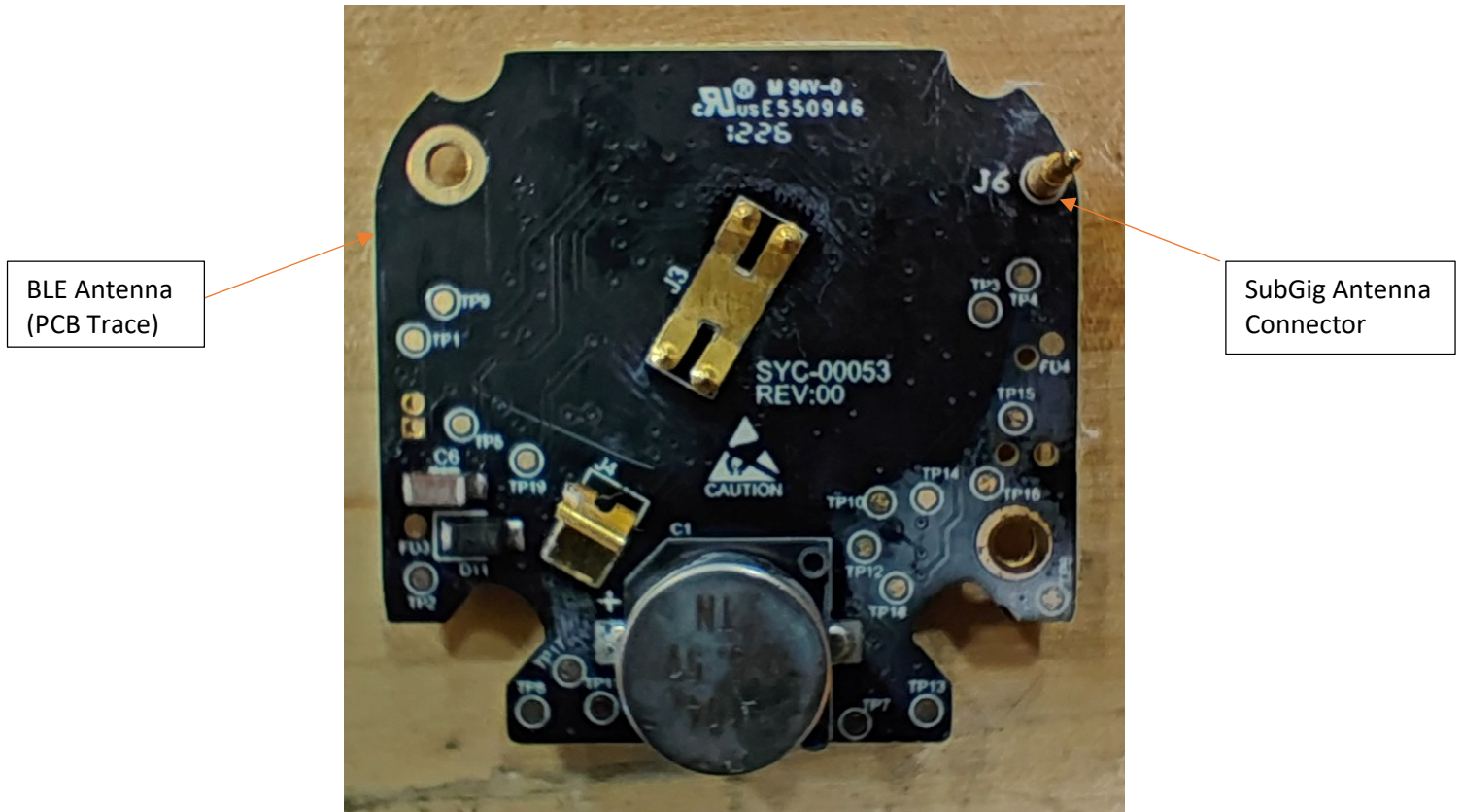
Figure 10 – PCB Back
