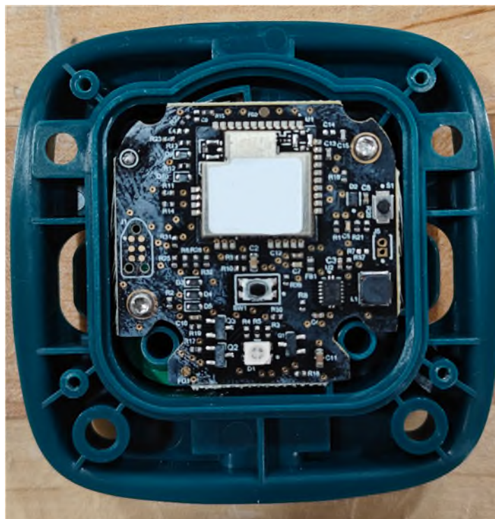
Figure 3 – Internal photo – Wall Button
