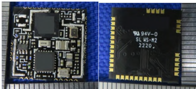
Figure 9 – Transmitter top and bottom, Shield Removed
