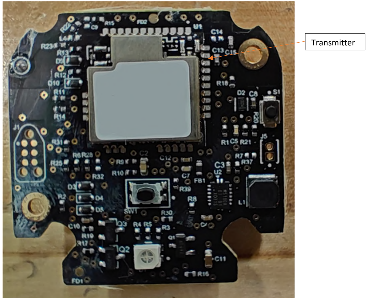
Figure 8 – PCB Front
