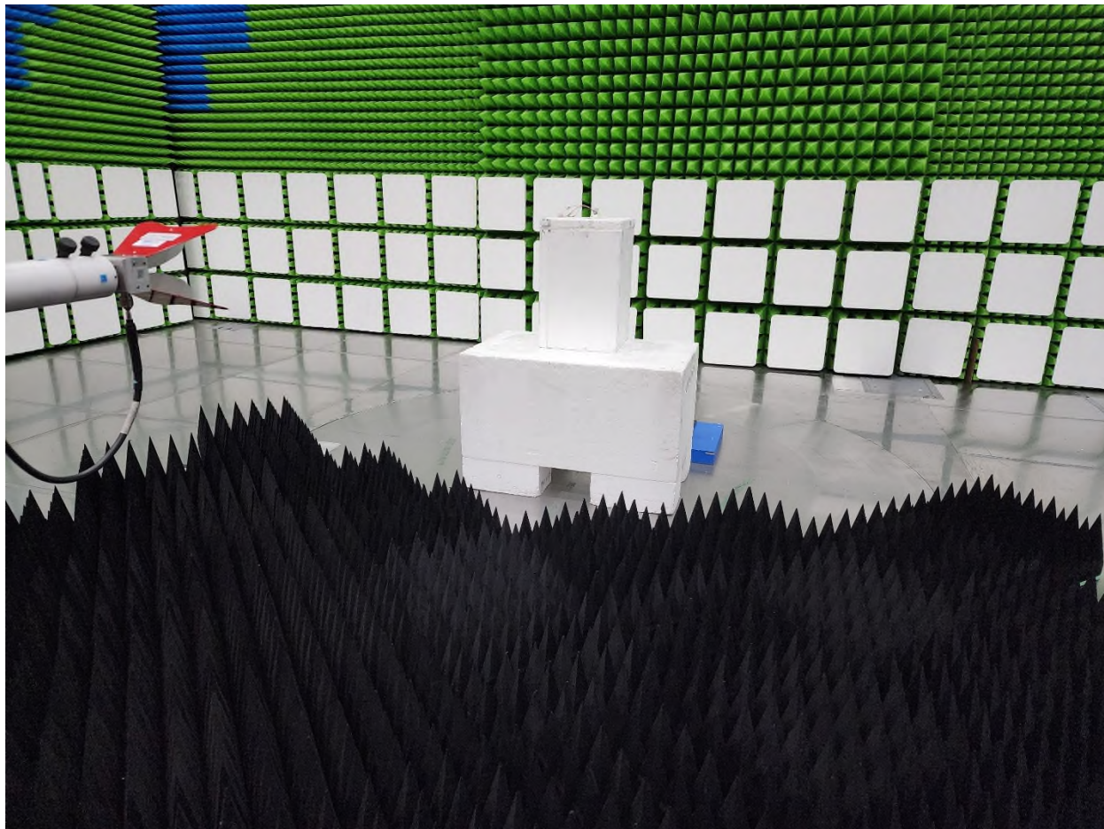
Figure 4 – Radiated Emissions Setup 1GHz – 18GHz
