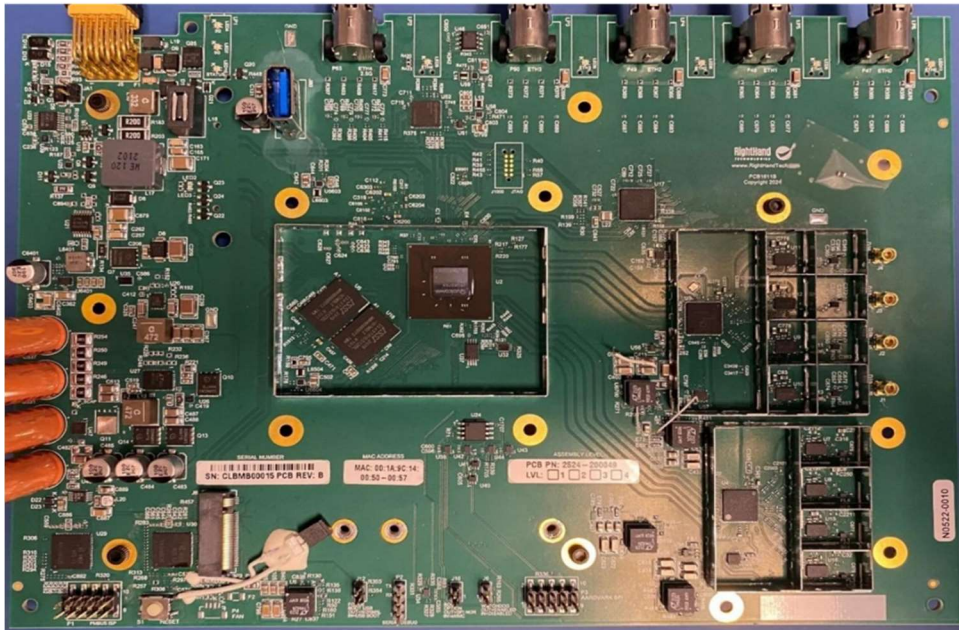
Figure 2-1: Main CPU board
