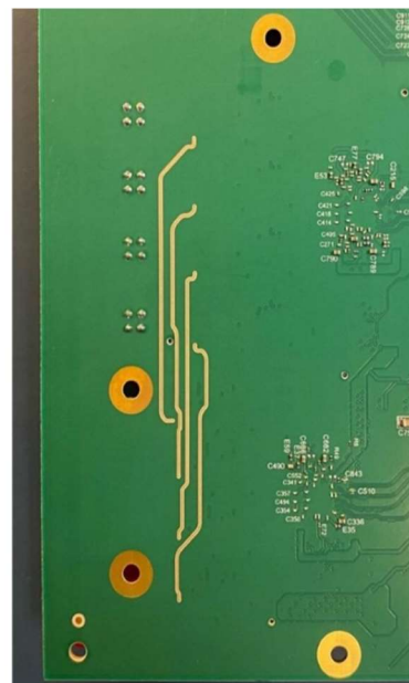
Figure 2-2: RF Front End Circuitry (Top – Left Side, Bottom – Right Side)
