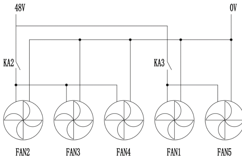
Figure 3.6.2 Fans' control diagram
