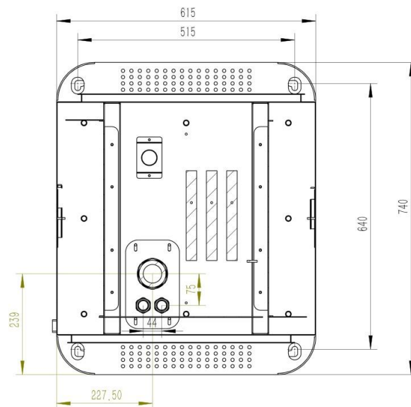
Figure 4.3.1 Concrete foundation for 150kW C6AM
