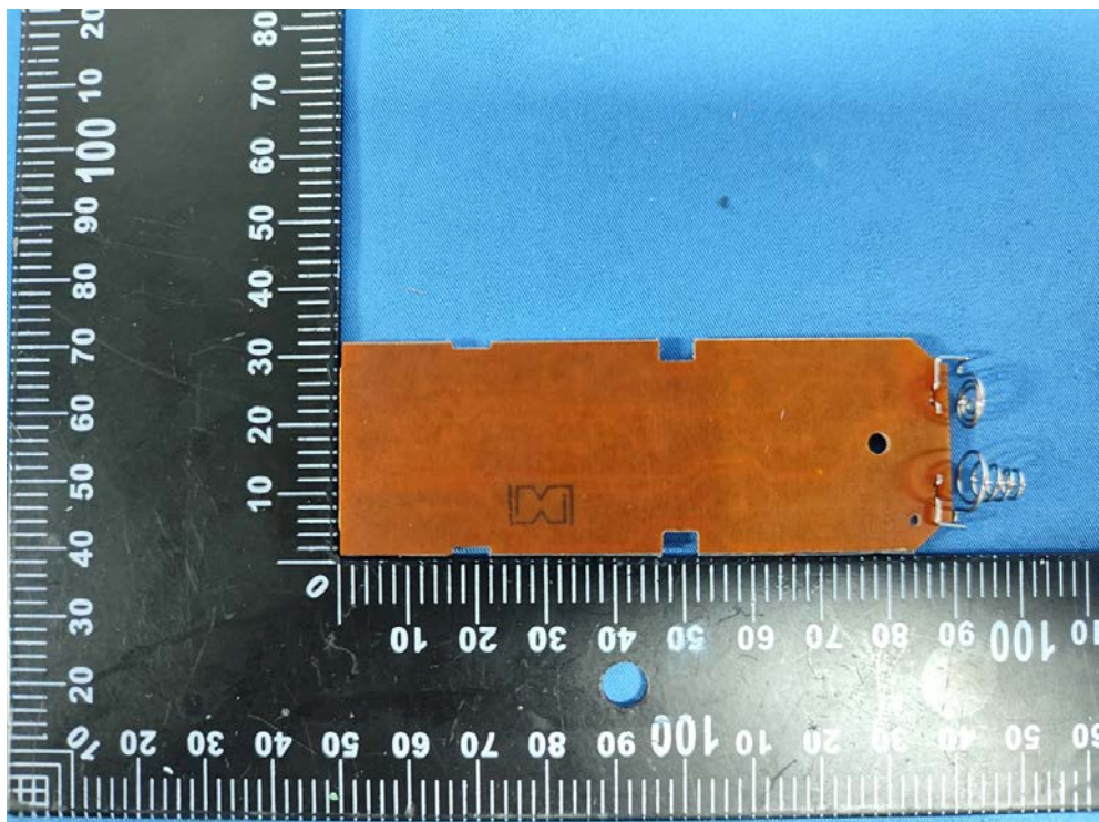
Antenna Location
