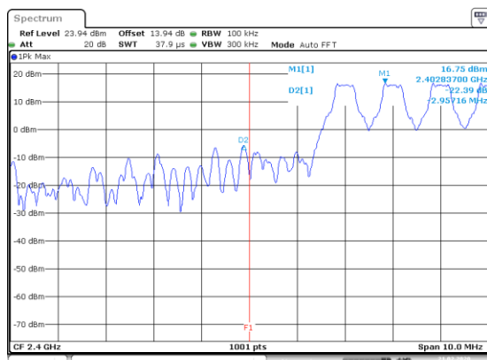
BR-1Mbps Hopping Left Side
