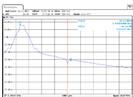
EDR-2Mbps Right Side
