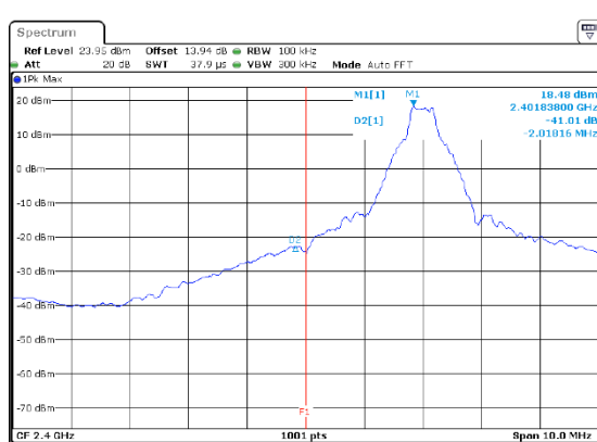
EDR-2Mbps Left Side
