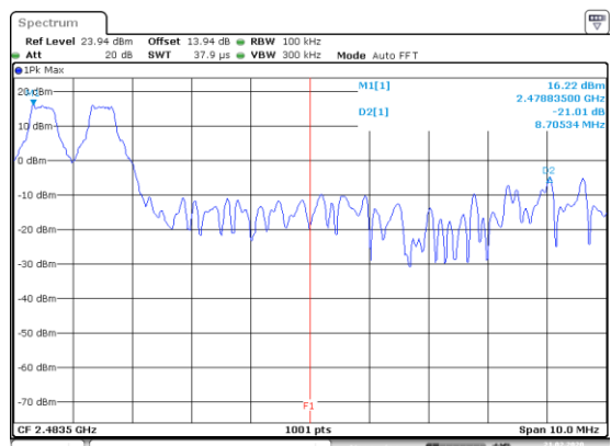
BR-1Mbps Hopping Right Side
