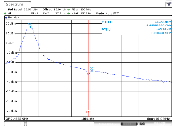
BR-1Mbps Right Side
