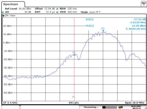
BLE-2Mbps Left Side
