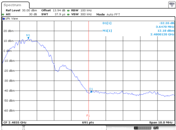
BLE-2Mbps Right Side
