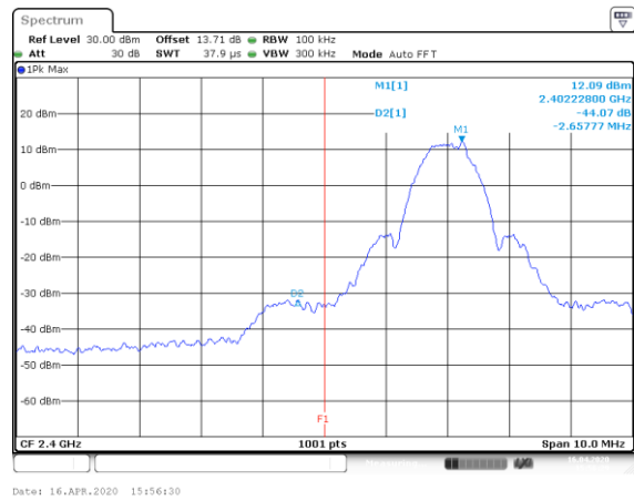
BLE-2Mbps Left Side
