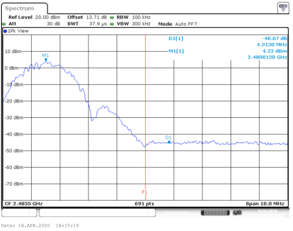
BLE-2Mbps Right Side
