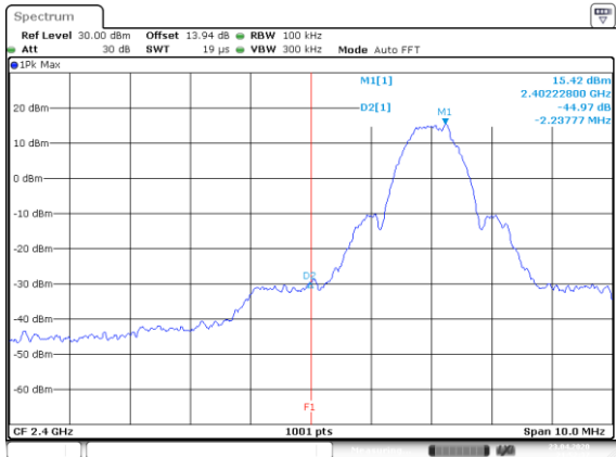
BLE-1Mbps Left Side
