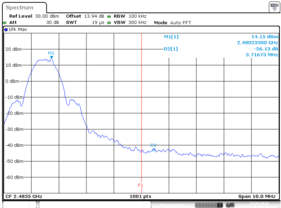
BLE-1Mbps Right Side
