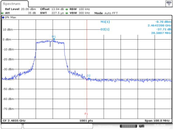
IEEE 802.11g Right Side
