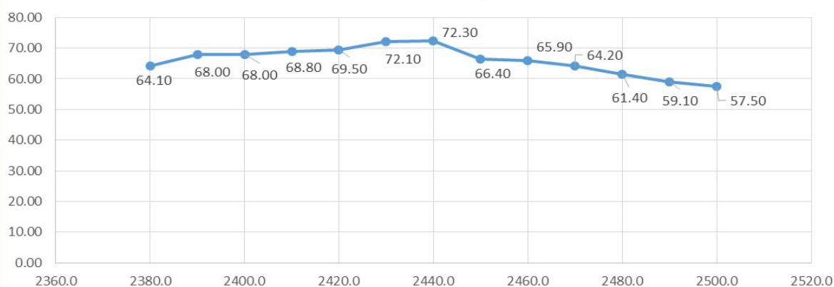
Efficiency (%)
