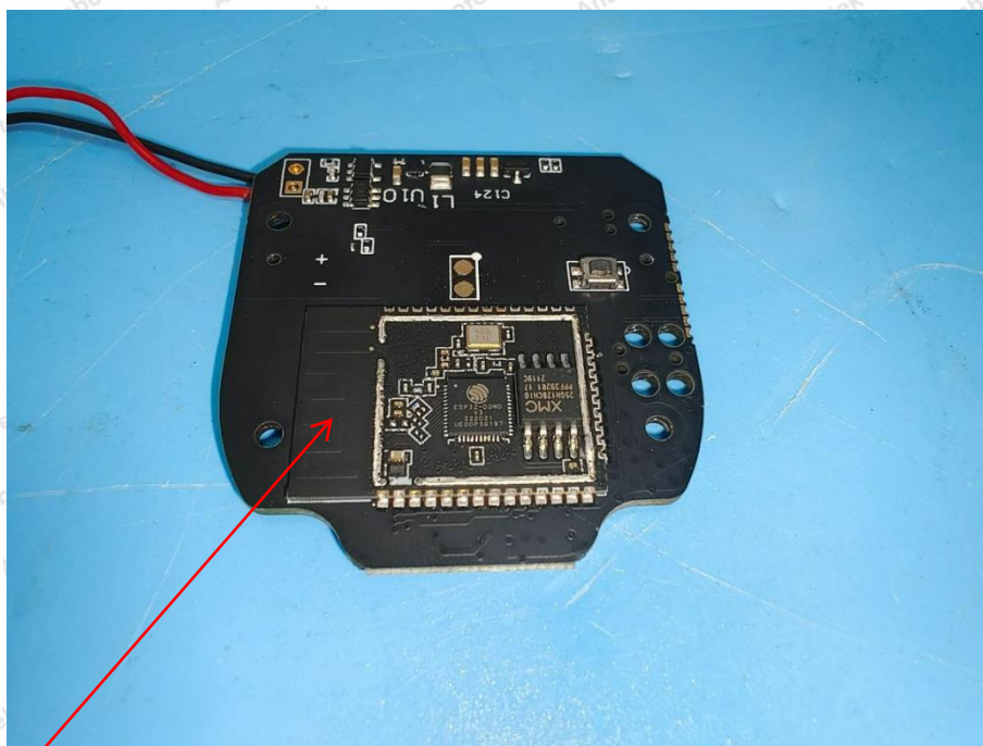
BT&WLAN ANT
