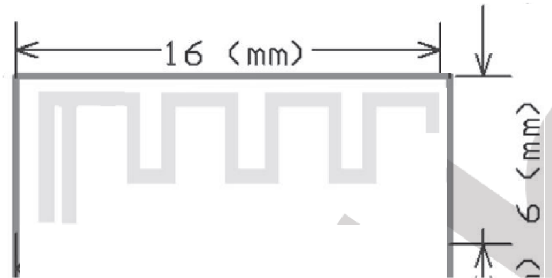
WIFI antenna
