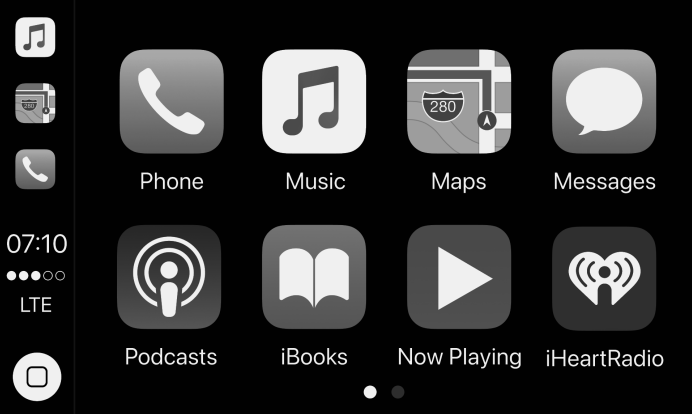
CarPlay interface
