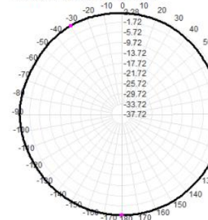
Total(H-XY), Max= 2.20dBi, CirD=1.48
