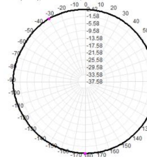
Total(H-XY), Max= 2.42dBi, CirD=1.25
