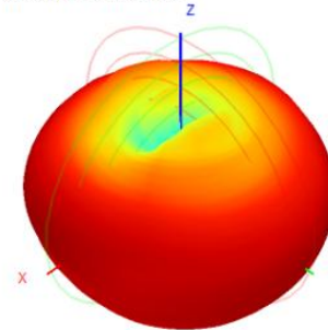
2450.0MHz H+V, Eff: 71.0%
