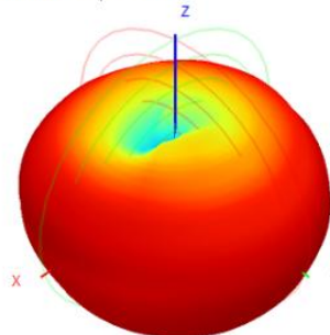
2400.0MHz H+V, Eff: 73.6%
