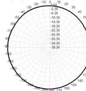
Total(H-XY), Max= 1.22dBi, CirD=1.82
