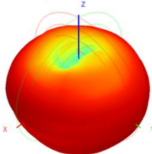
2500.0MHz H+V, Eff: 61.0%
