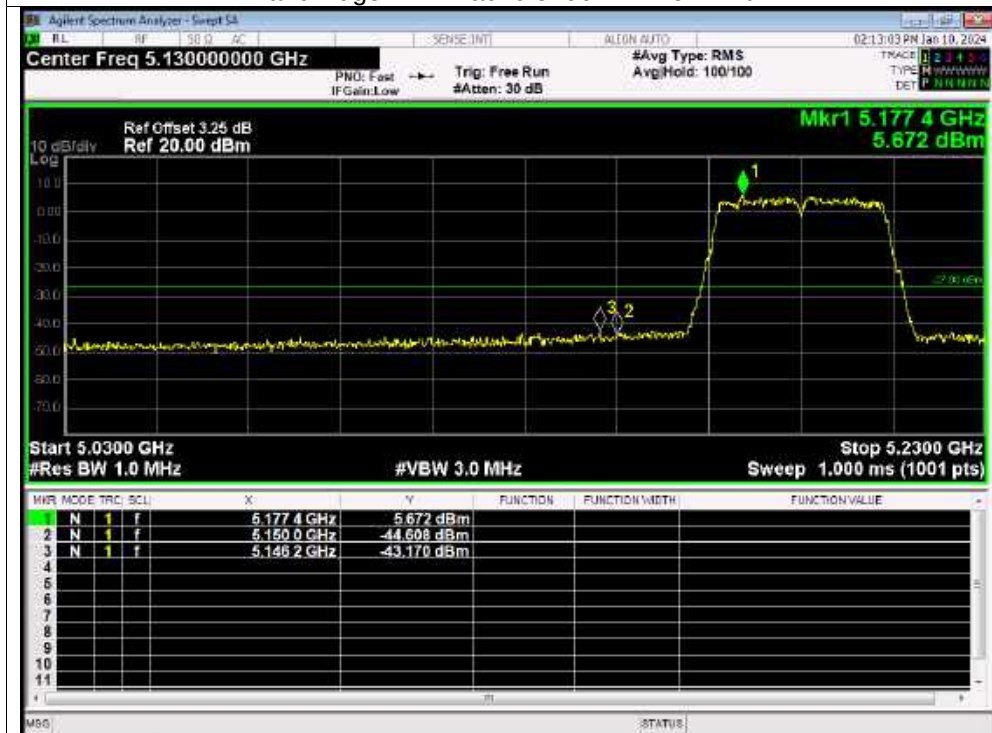
Band Edge NVNT ac40 5190MHz Low Ant1
