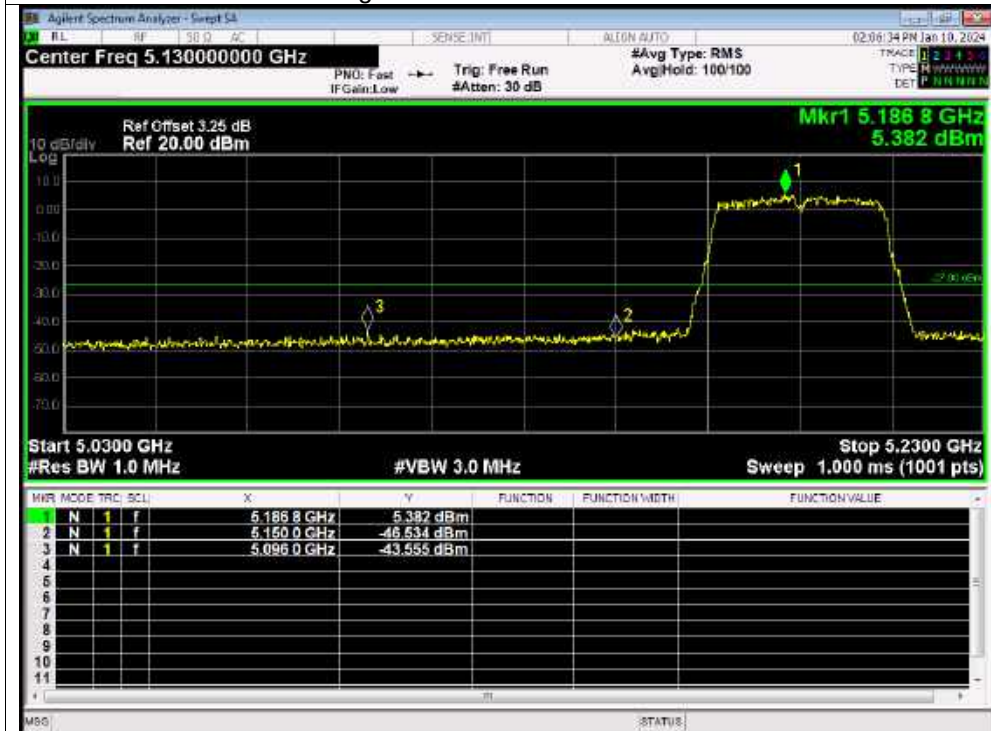
Band Edge NVNT n40 5190MHz Low Ant1
