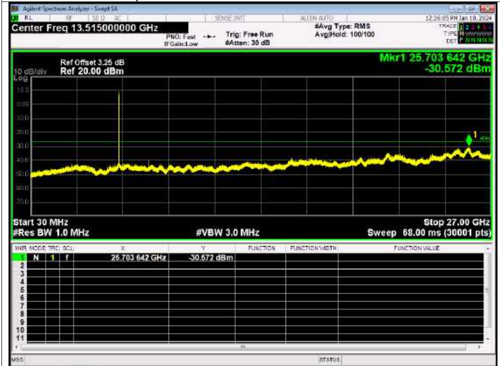
Tx. Spurious NVNT ac20 5200MHz Ant1 Emission
