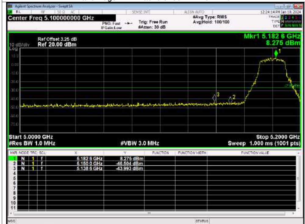
Band Edge NVNT ac20 5180MHz Low Ant1
