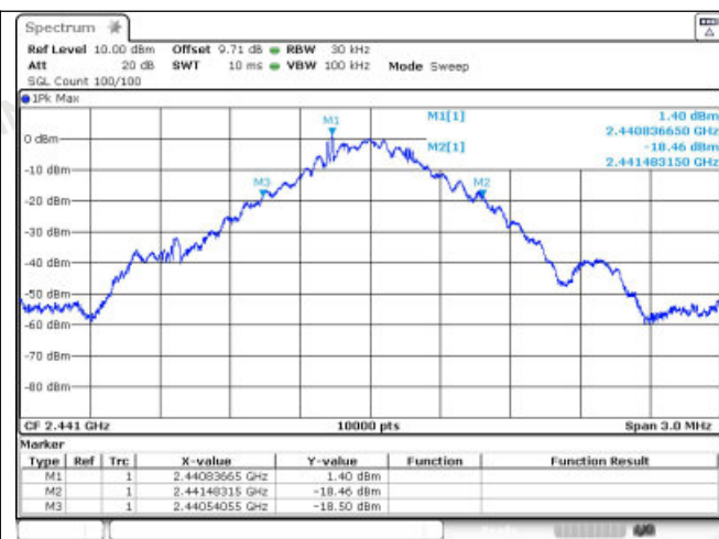
GFSK_DH5_Channel 39
