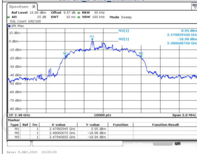
8DPSK_3-DH5_Channel 78
