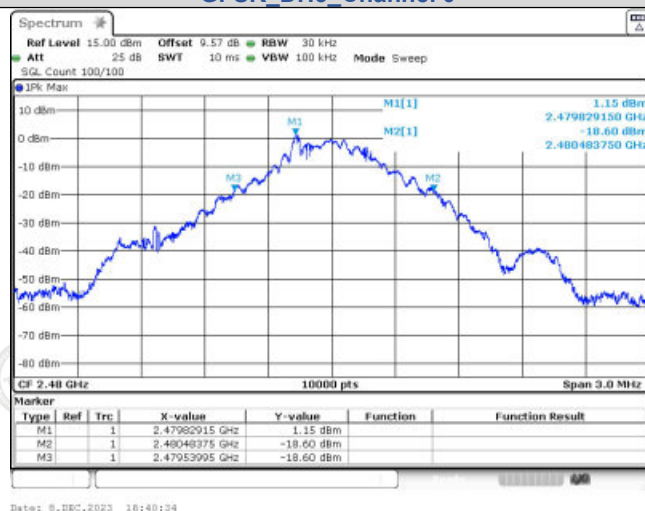
GFSK_DH5_Channel 78
