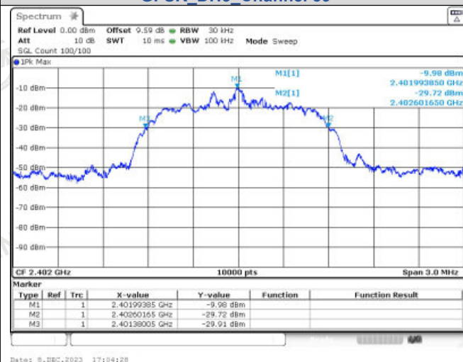
\pi/4 DQPSK_2-DH5_Channel 0
