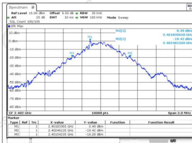
GFSK_DH5_Channel 0
