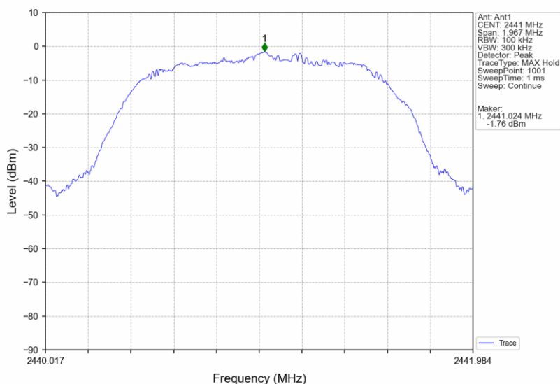
8DPSK_3DH5_MCH_2441MHz_Ant1_NTNV
