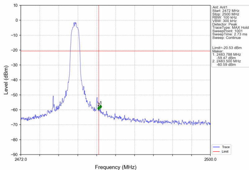
Pi/4DQPSK_2DH5_HCH_2480MHz_Ant1_NTNV
