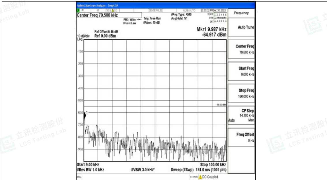
Band7_10MHz_QPSK_21400_1RB#0_0.009~0.15_0.009~0.15
