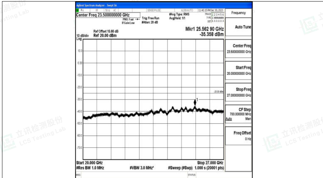
Band7_15MHz_QPSK_20825_1RB#0_20000~27000_20000~27000
