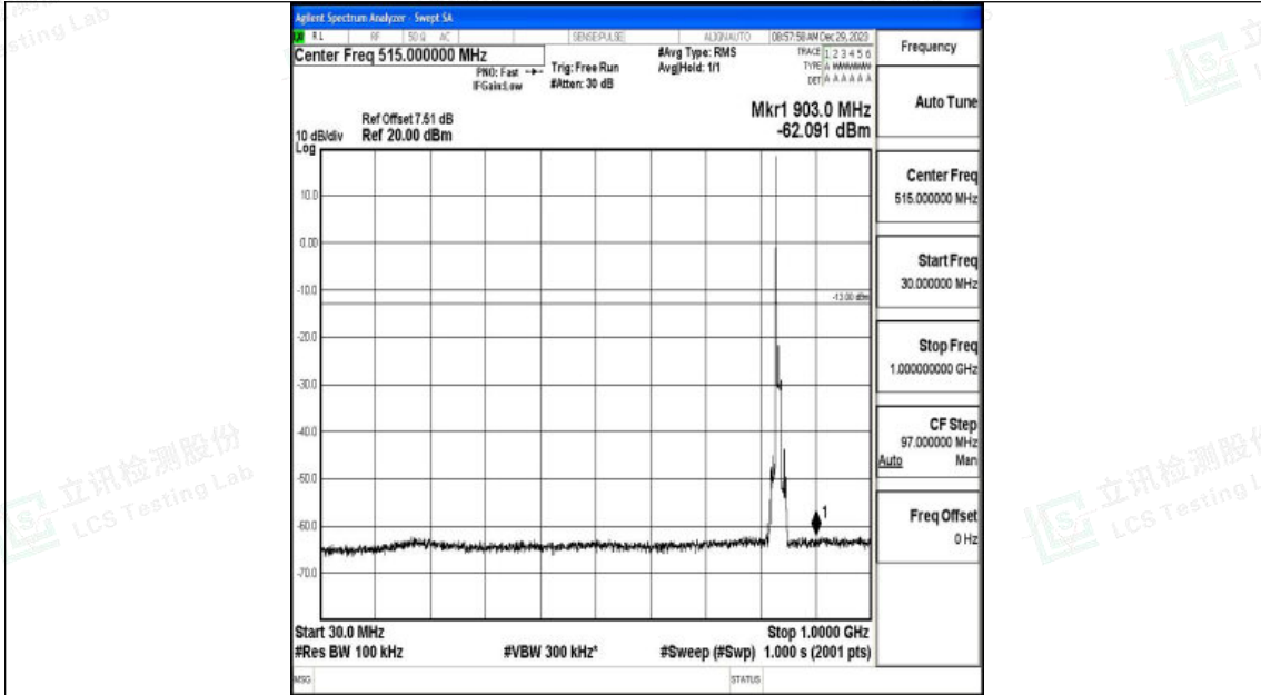
Band26_10MHz_QPSK_26915_1RB#0_30~1000_30~1000
