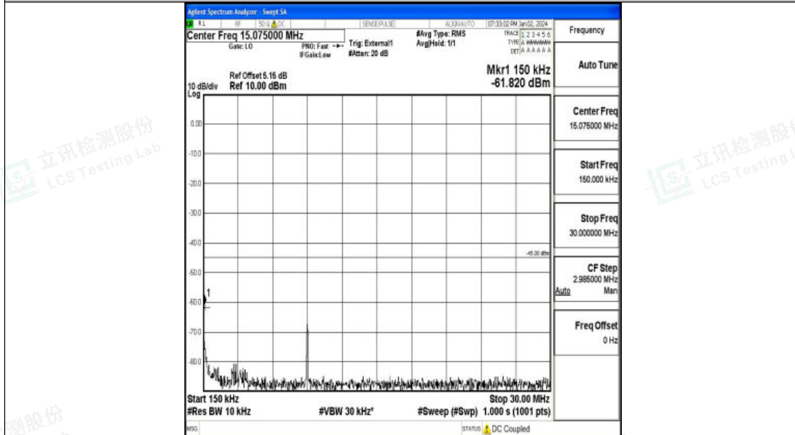
Band38_5MHz_QPSK_37775_1RB#0_0.15~30_0.15~30
