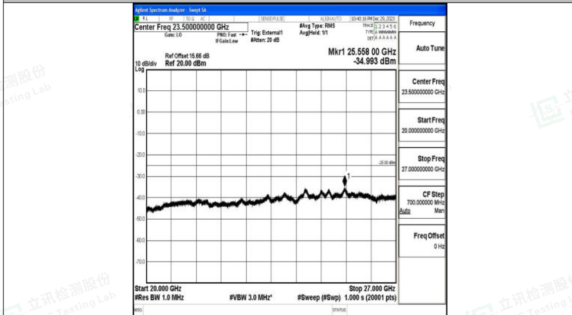
Band41_15MHz_16QAM_39725_1RB#0_20000~27000_20000~27000
