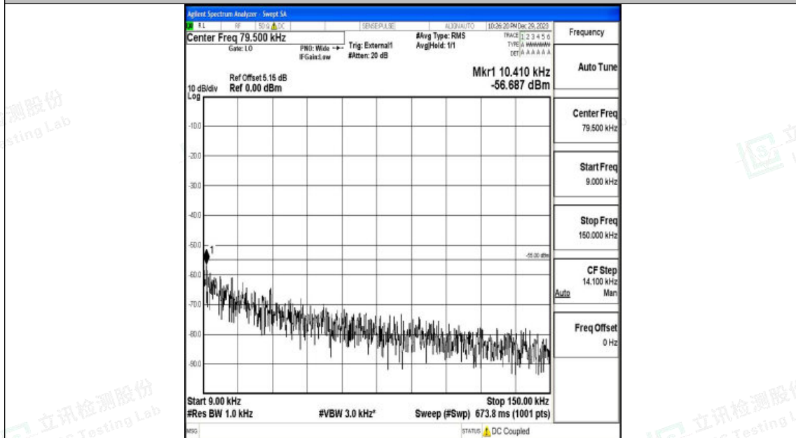
Band41_10MHz_QPSK_41540_1RB#0_0.009~0.15_0.009~0.15
