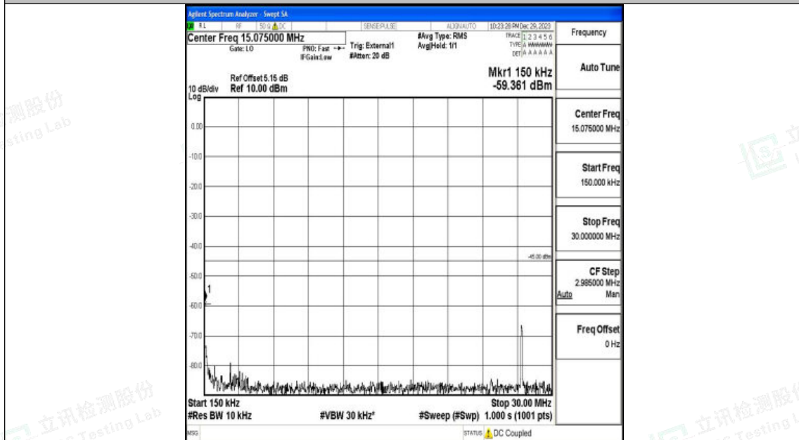
Band41_10MHz_QPSK_40620_1RB#0_0.15~30_0.15~30
