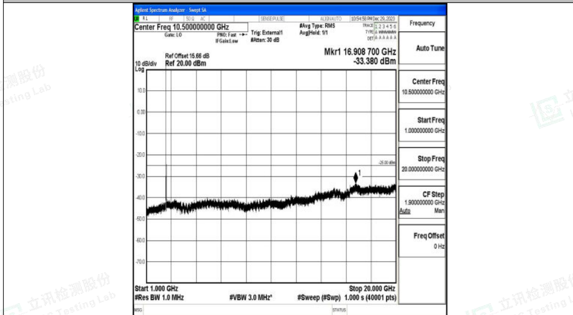
Band41_20MHz_16QAM_39750_1RB#0_1000~20000_1000~20000
