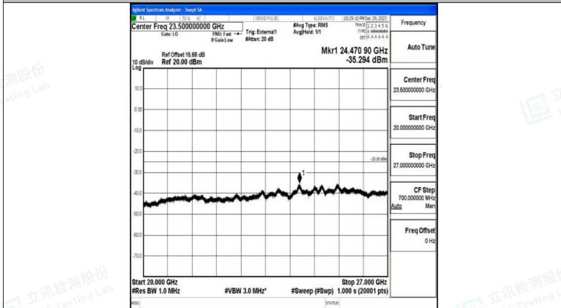
Band41_10MHz_16QAM_41540_1RB#0_20000~27000_20000~27000
