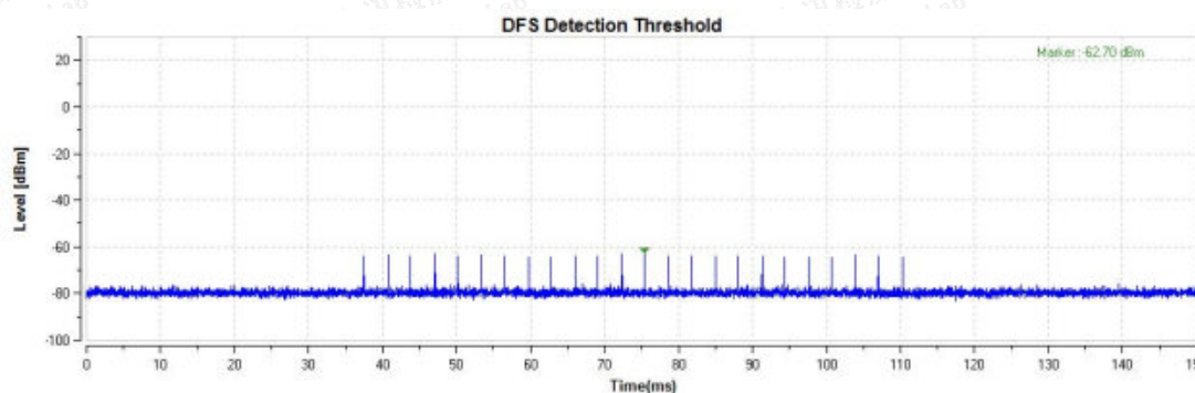
Radar Singal 5
