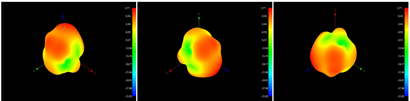
3D 2450:
