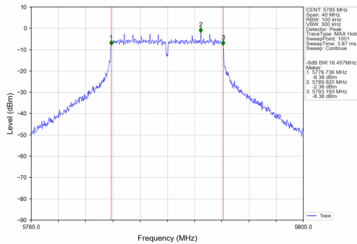
802.11a_MCH_5785MHz_Ant1_NTN
