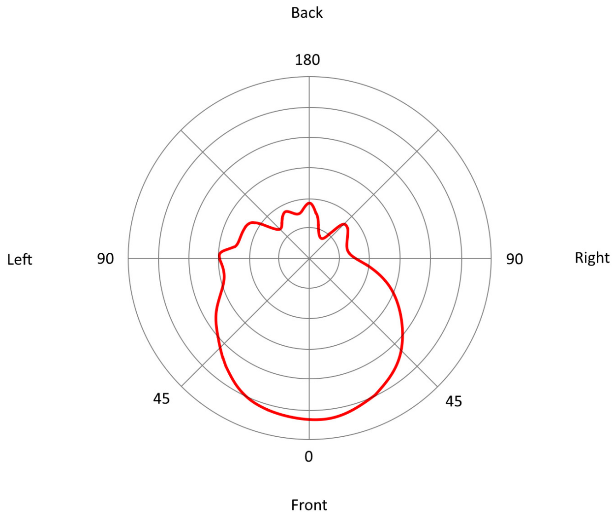
Bluetooth Signal Relative Strength
