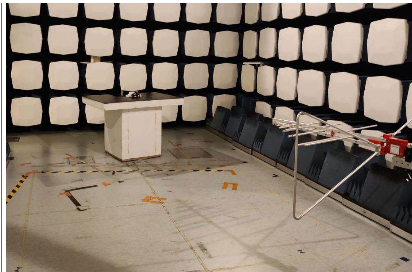
Picture 13, Radiated Spurious Emissions, common setup, TX and RX 30 - 1000 MHz
