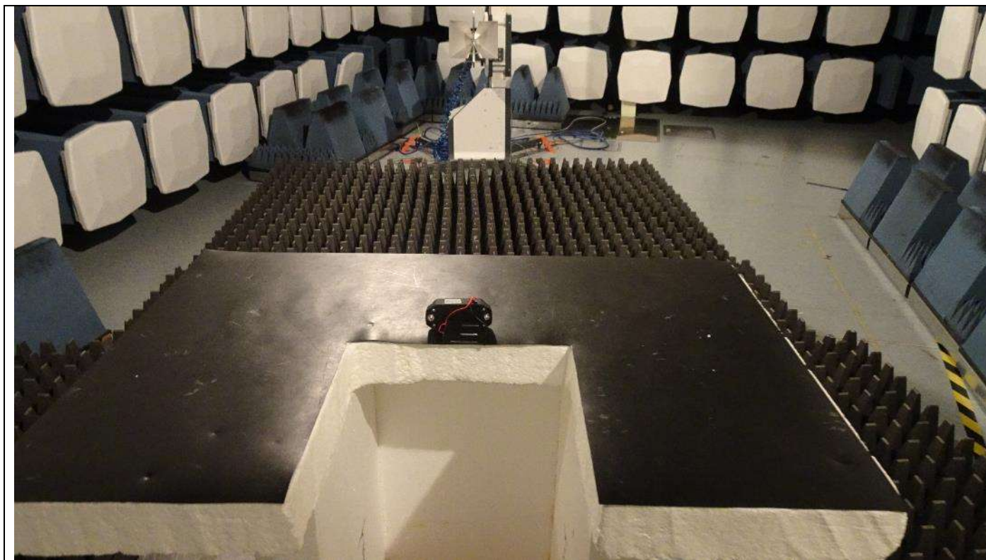
Picture 19, Radiated Spurious Emissions, EUT setup, RX 1 – 18 GHz, back view
