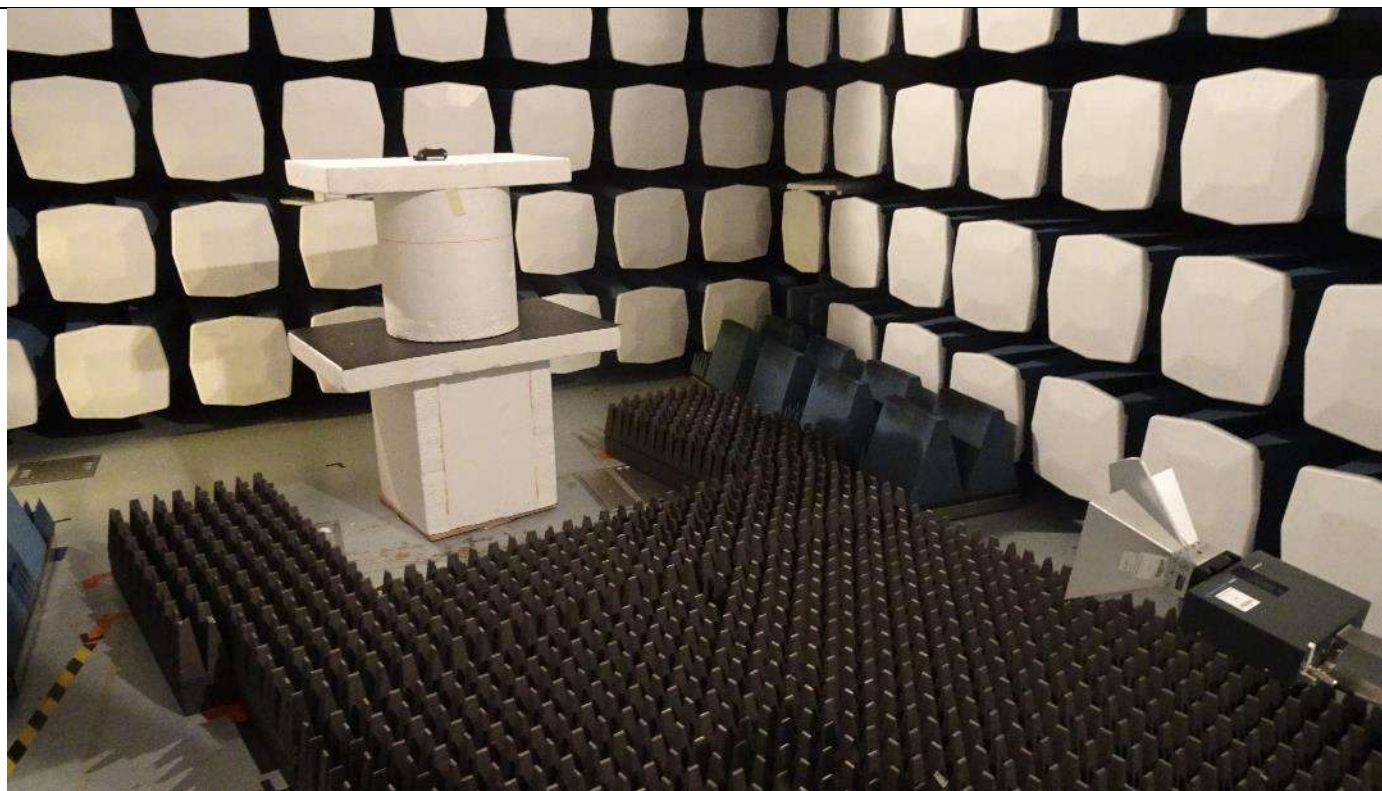
Picture 14, Radiated Spurious Emissions, common setup, TX, 1 – 26 GHz
