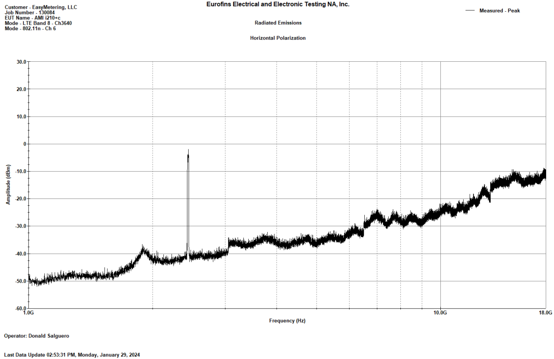
Figure 33. Colocation Radiated Emissions_LTE B8_WiFi ch6_1-18GHz_H
