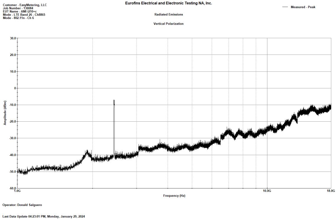
Figure 14. Colocation Radiated Emissions_LTE B26_WiFi ch6_1-18GHz_V
