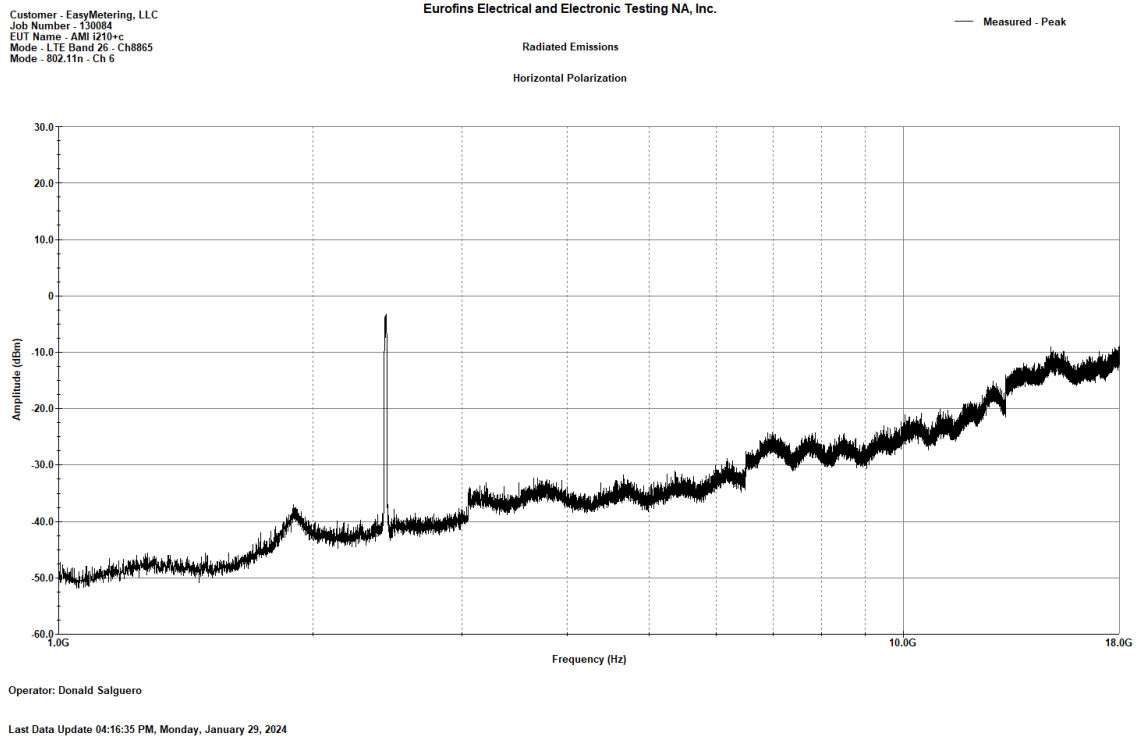
Figure 13. Colocation Radiated Emissions_LTE B26_WiFi ch6_1-18GHz_H
