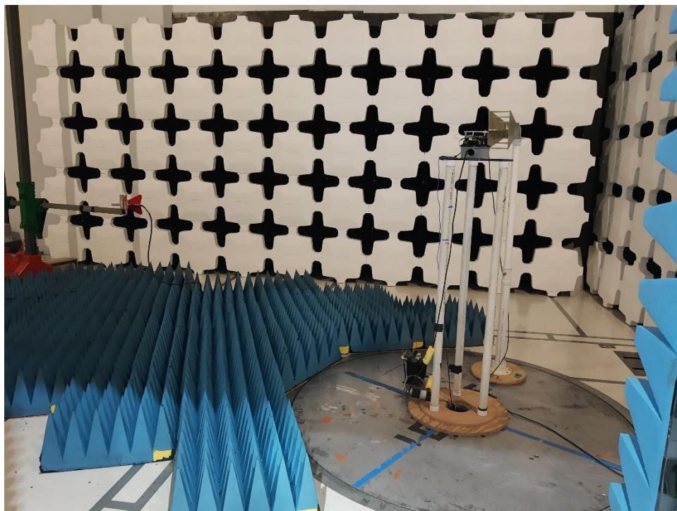
Photograph 2. RE Setup [1GHz - 18GHz]
