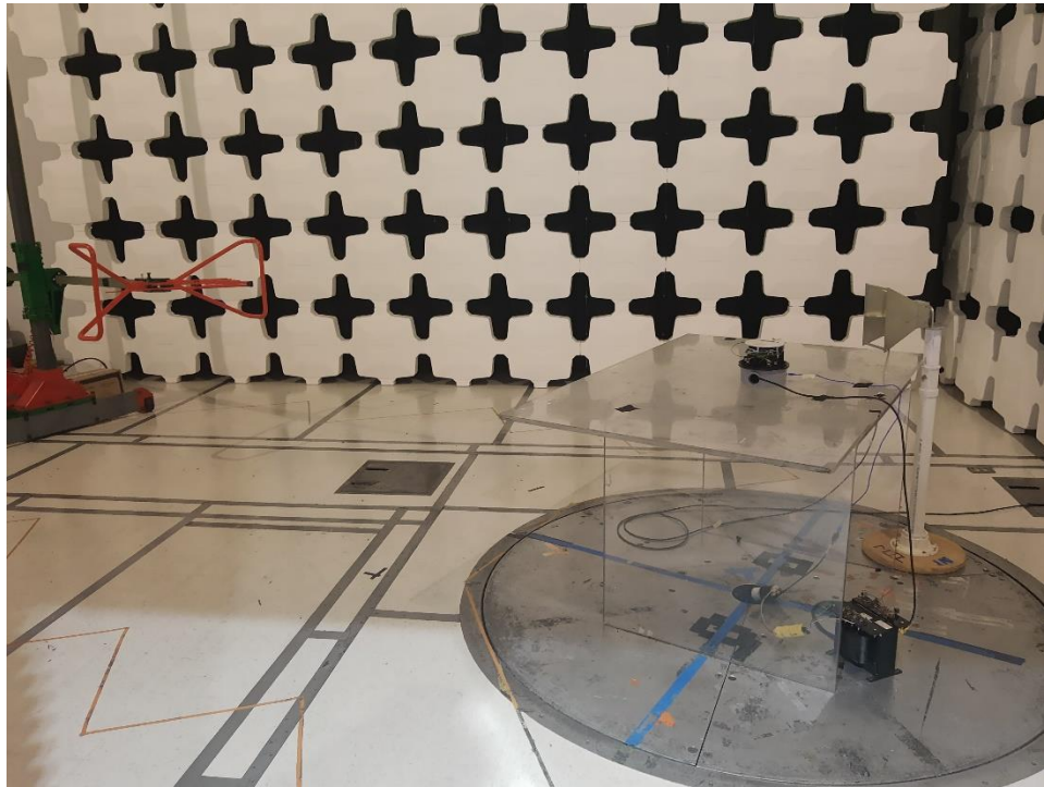
Photograph 1. RE Setup [30MHz - 1GHz]
