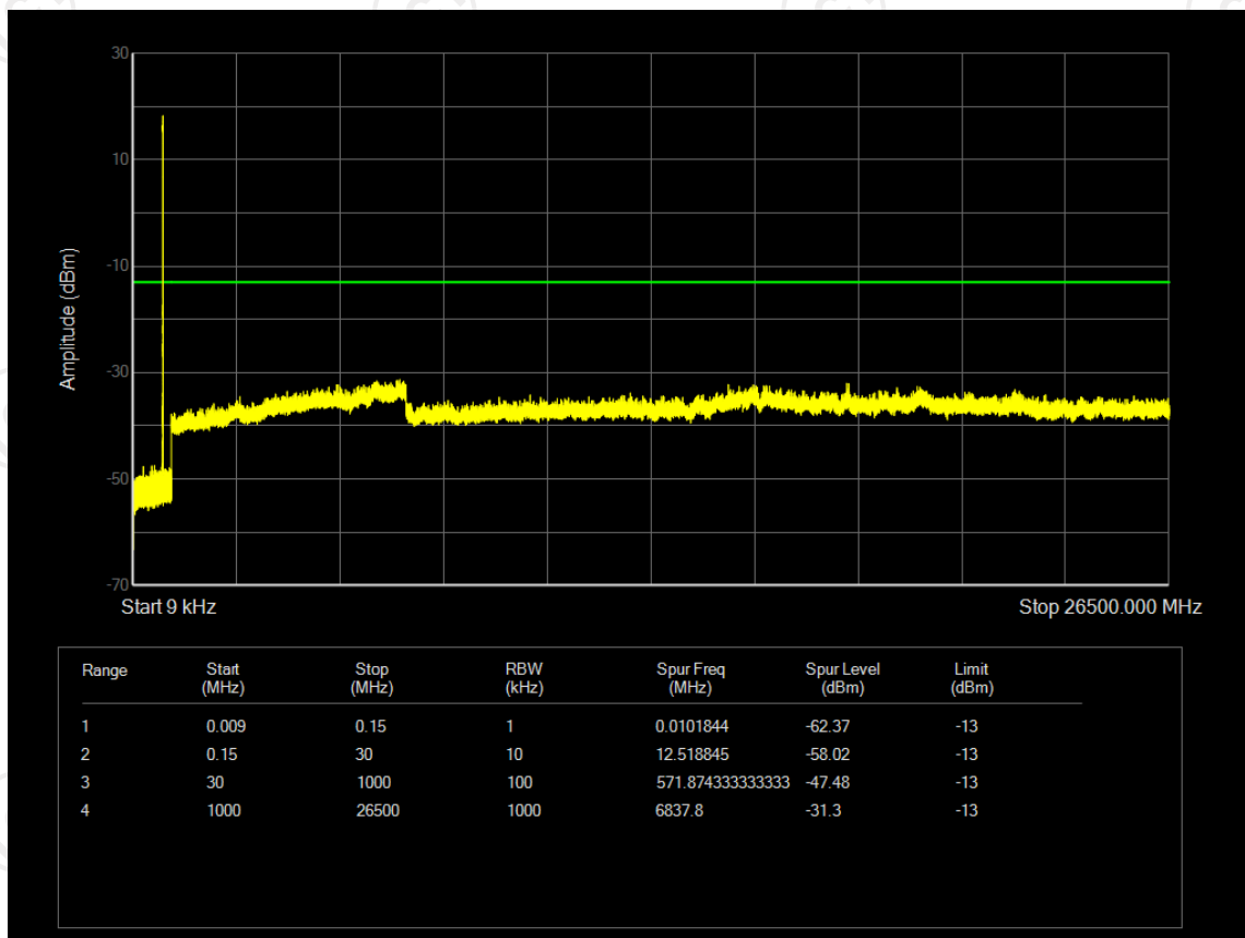
Band26(824-849) 16QAM BW=3MHz Channel=26805 RB Size=15 Position=#0
