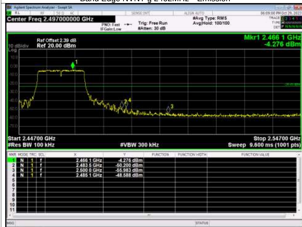
Band Edge NVNT g 2462MHz Emission
