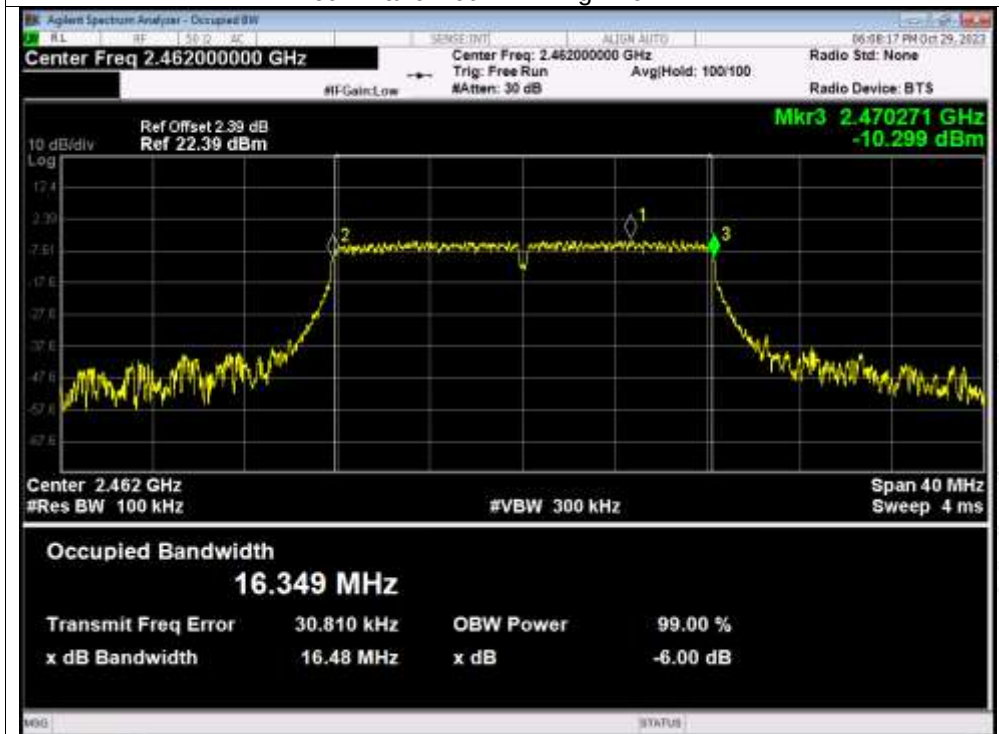
-6dB Bandwidth NVNT g 2462MHz
