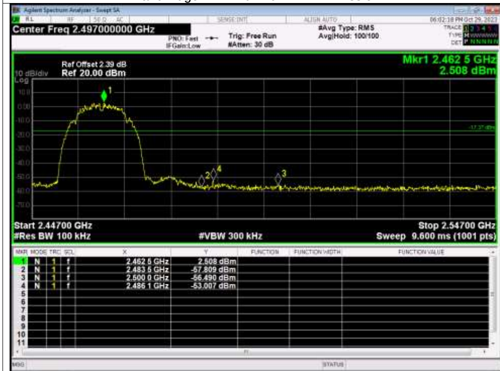
Band Edge NVNT b 2462MHz Emission
