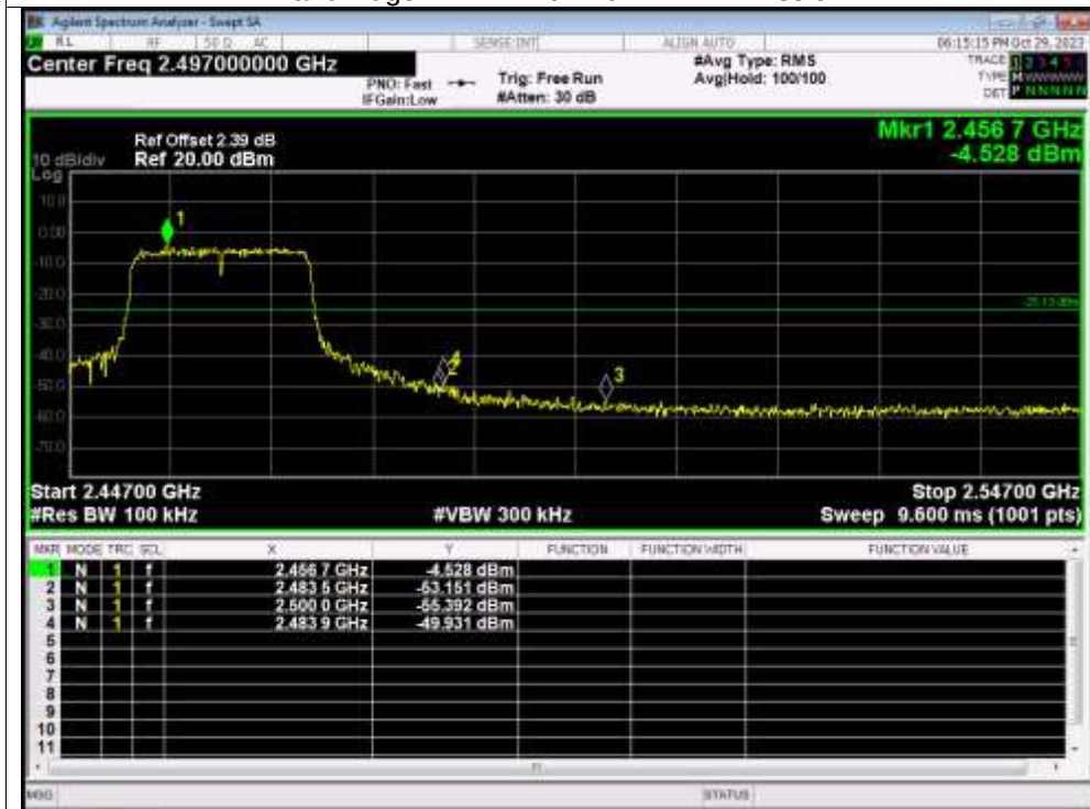
Band Edge NVNT n20 2462MHz Emission
