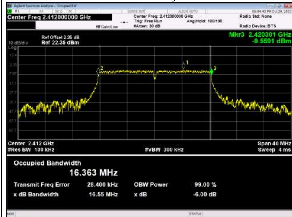
-6dB Bandwidth NVNT g 2412MHz
