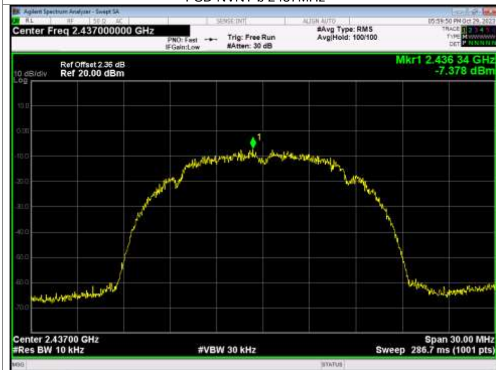
PSD NVNT b 2437MHz
