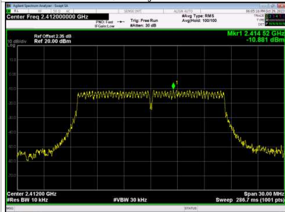
PSD NVNT g 2412MHz
