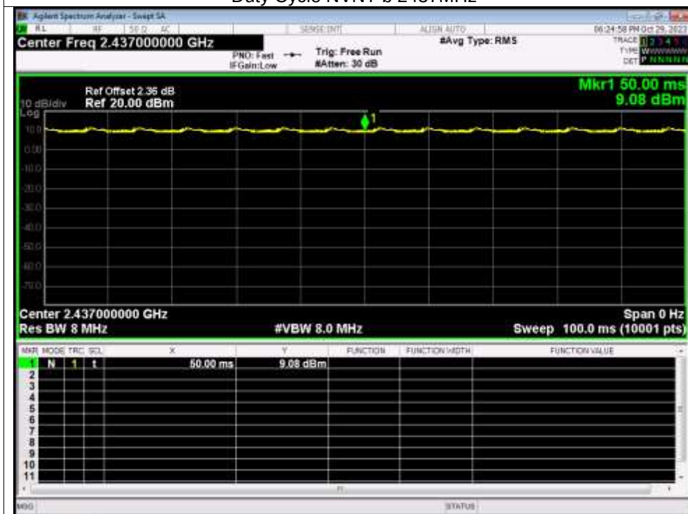
Duty Cycle NVNT b 2437MHz
