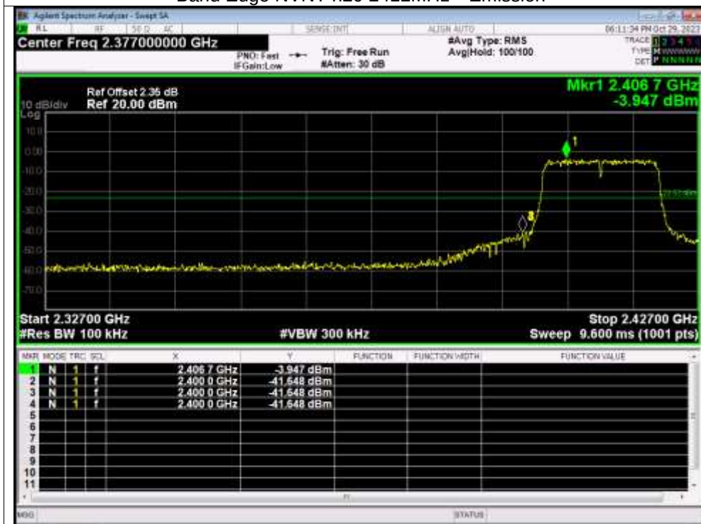
Band Edge NVNT n20 2412MHz Emission
