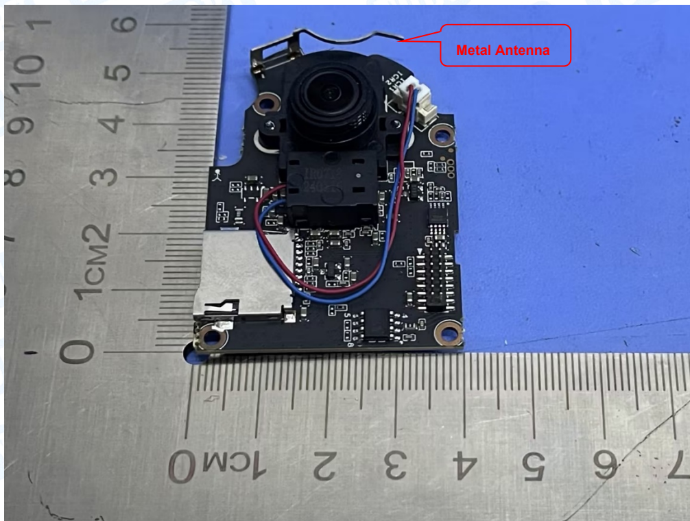
Photo 12 Appearance of PCB 1#
