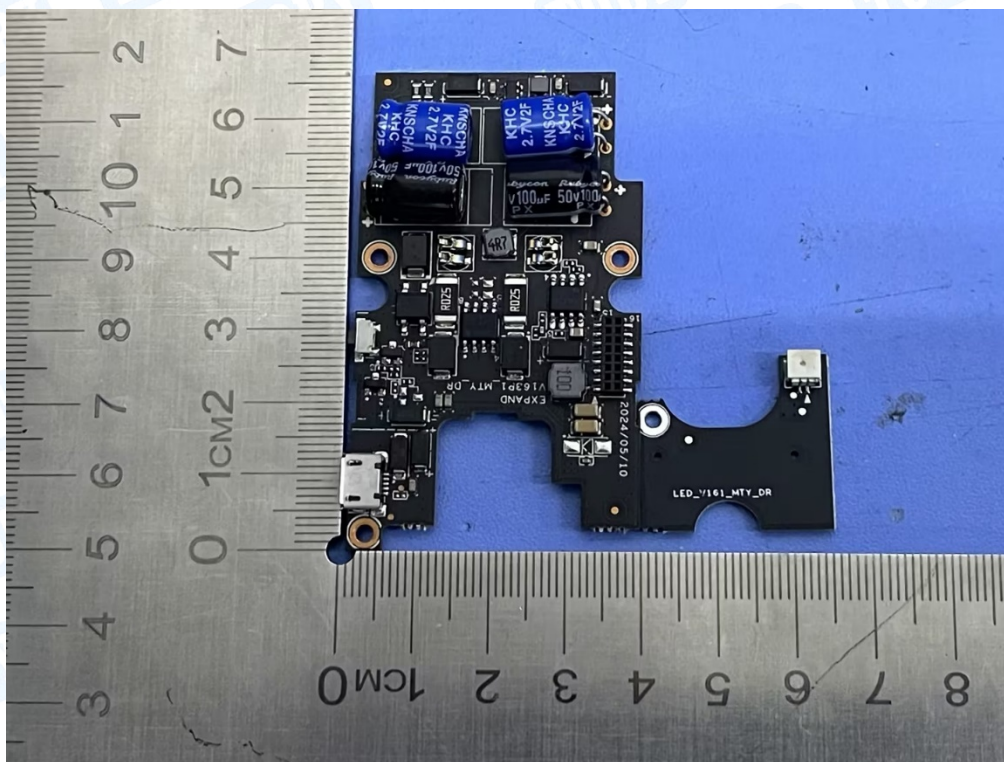
Photo 15 Appearance of PCB 2#
