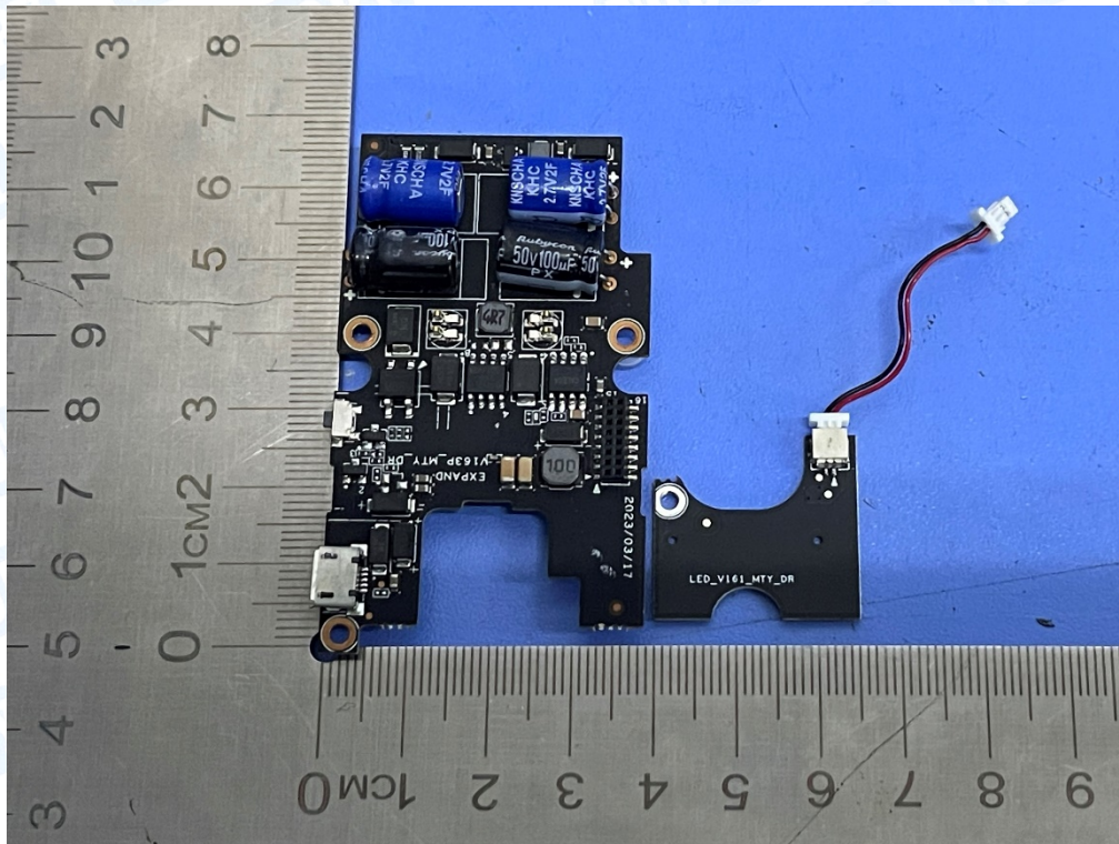
Photo 14 Appearance of PCB 2#
