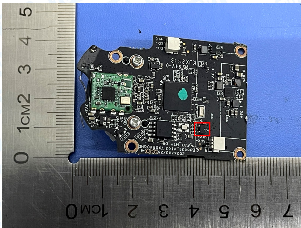
Photo 10 Appearance of PCB 2#
