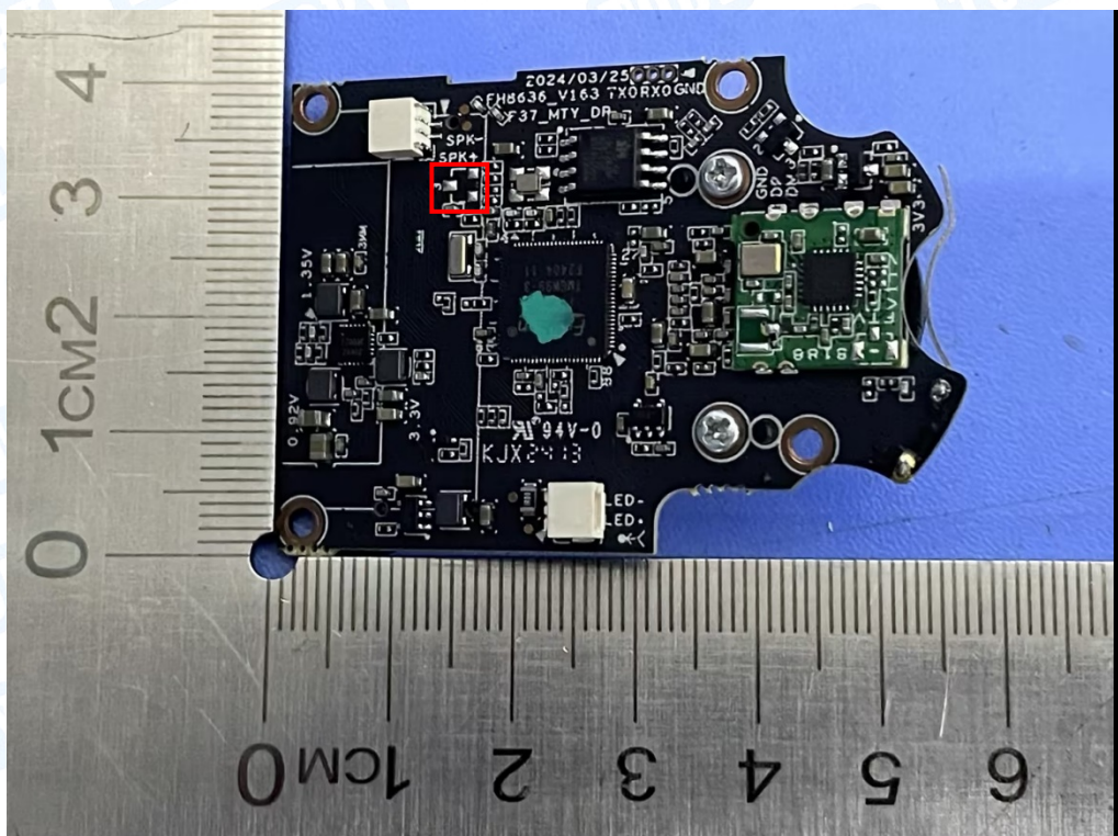
Photo 10 Appearance of PCB 2#
