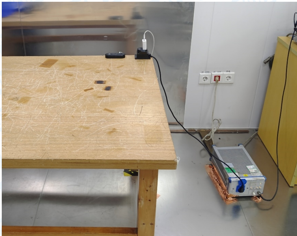
Photo of Setup for Radiated Emission (30MHz~1GHz)
