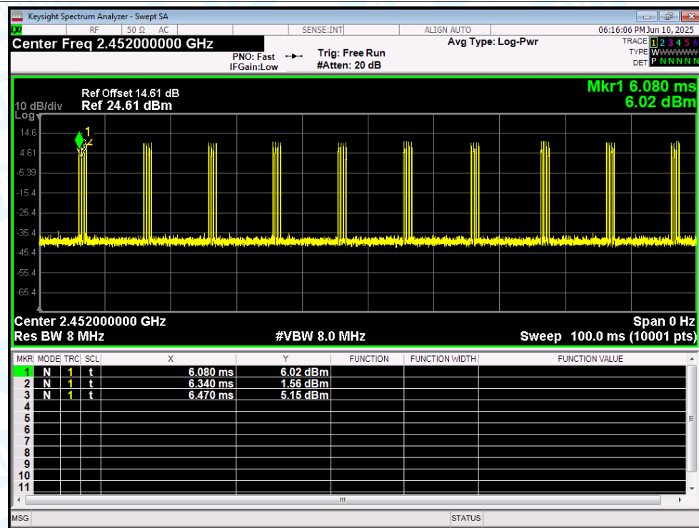
Duty Cycle NVNT n(HT40) 2452MHz Sum
