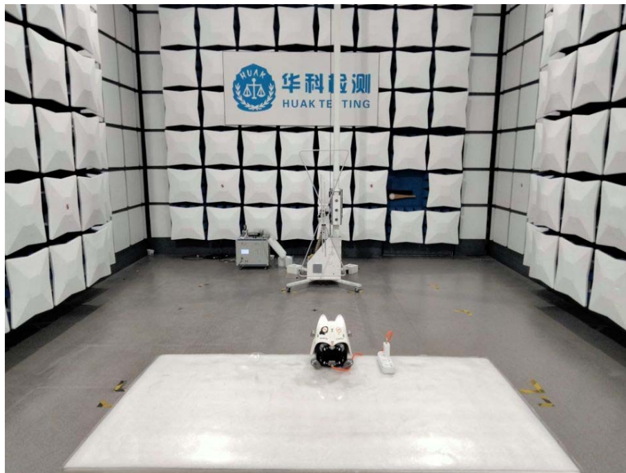
Model: M-Y-DSM1 Radiated Emissions
