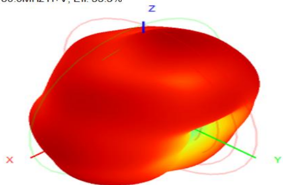
780.0MHz H+V, Eff. 33.3%
