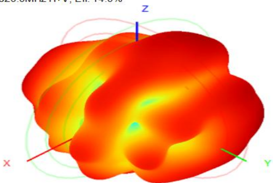
2620.0MHz H+V, Eff. 14.0%
