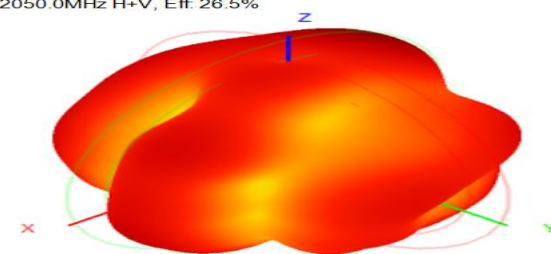
2050.0MHz H+V, Eff. 26.5%
