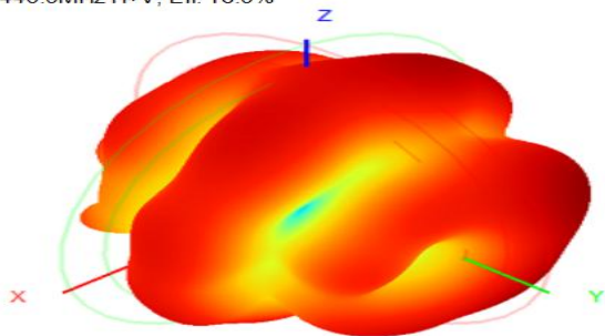
2440.0MHz H+V, Eff. 16.0%
