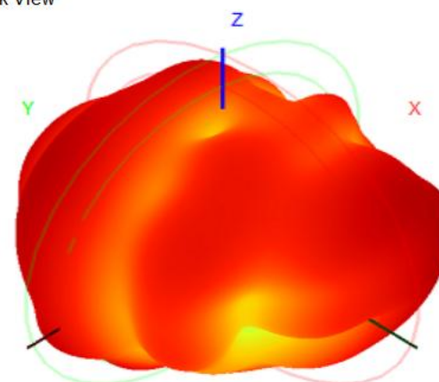
Back View
