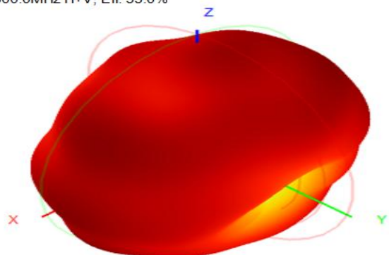
800.0MHz H+V, Eff. 33.0%
