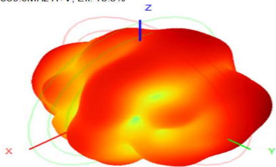
2580.0MHz H+V, Eff. 13.8%
