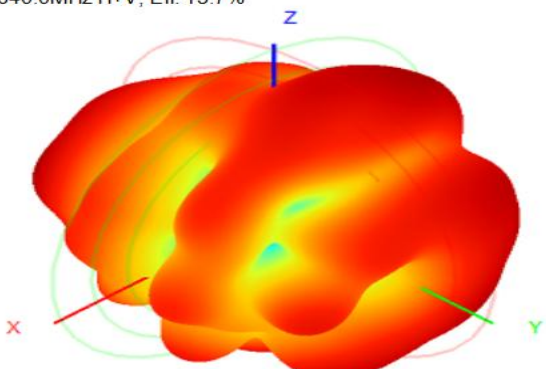
2640.0MHz H+V, Eff. 13.7%
