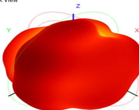
Back View
