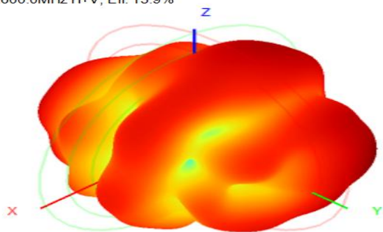
2600.0MHz H+V, Eff. 13.9%
