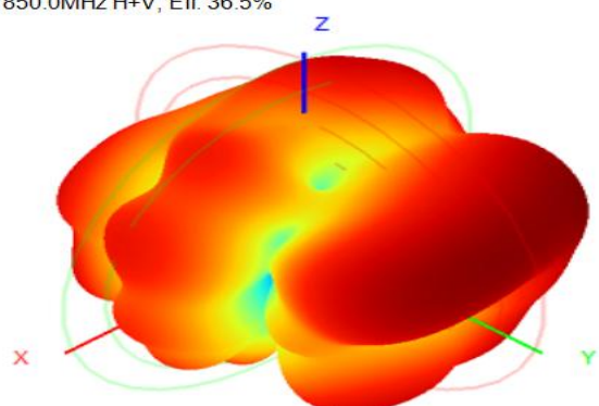
1850.0MHz H+V, Eff. 36.5%
