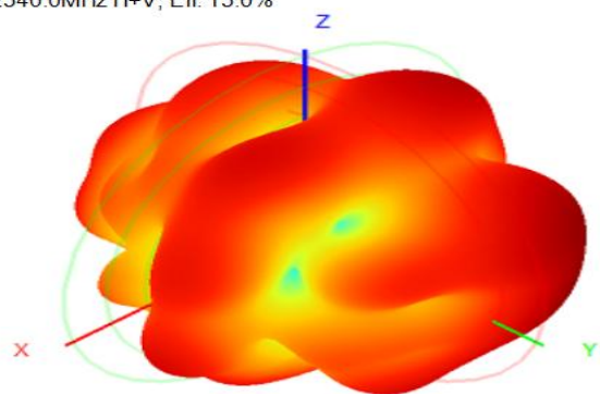
2540.0MHz H+V, Eff: 15.0%
