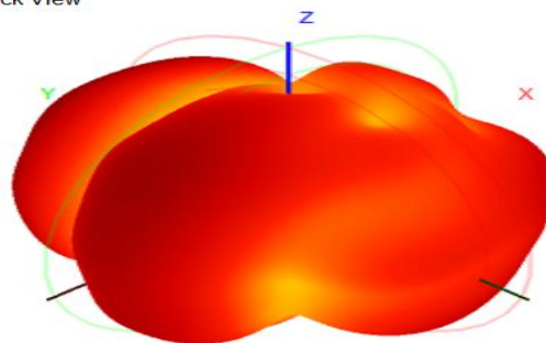
Back View
