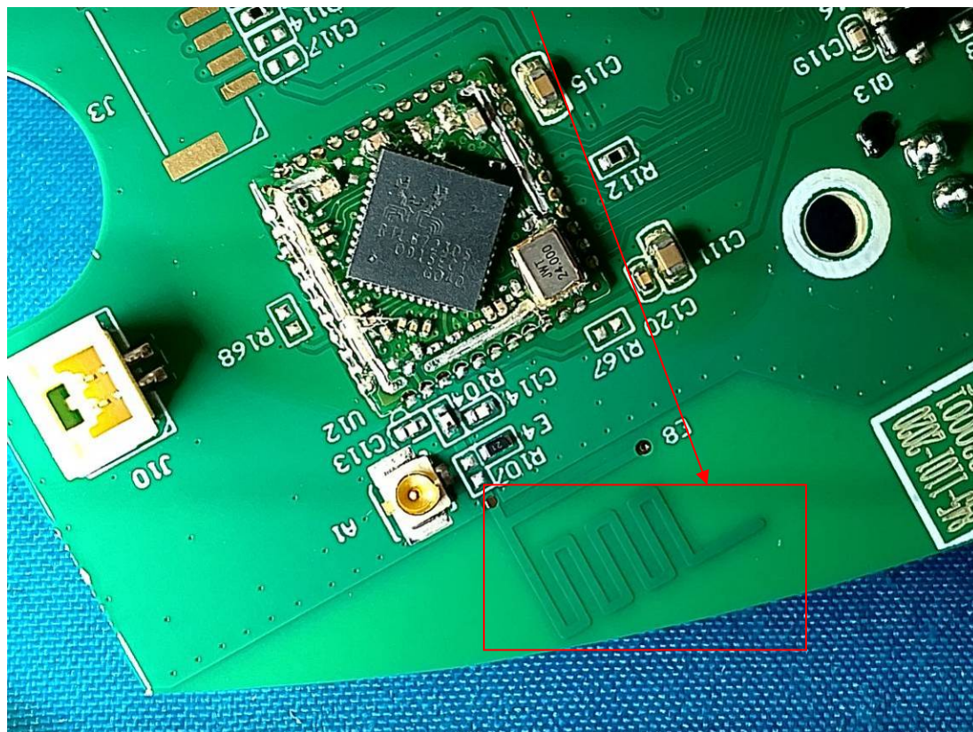
Antenna(no use)
