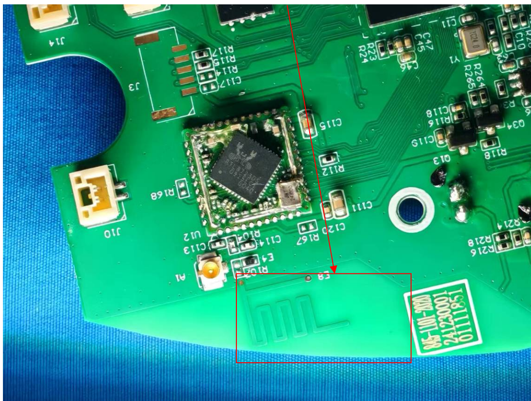
Antenna(no use)
