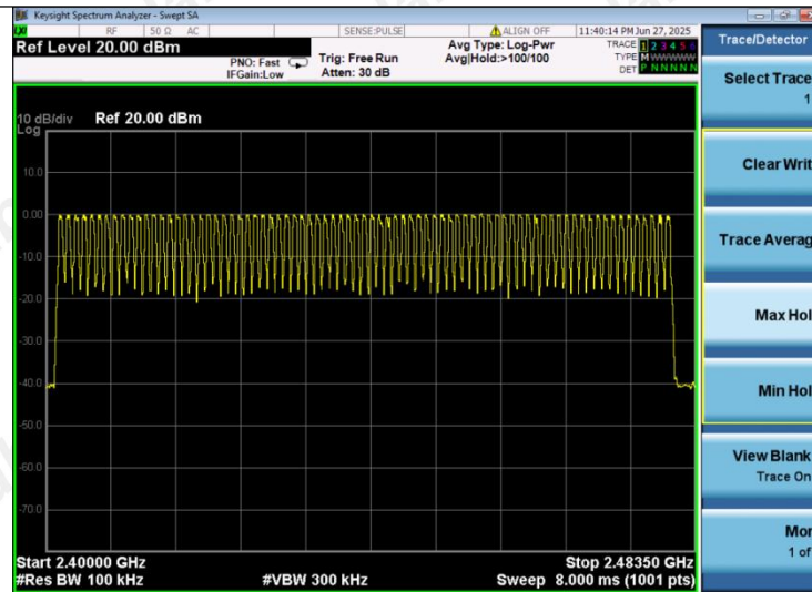
GFSK Modulation
