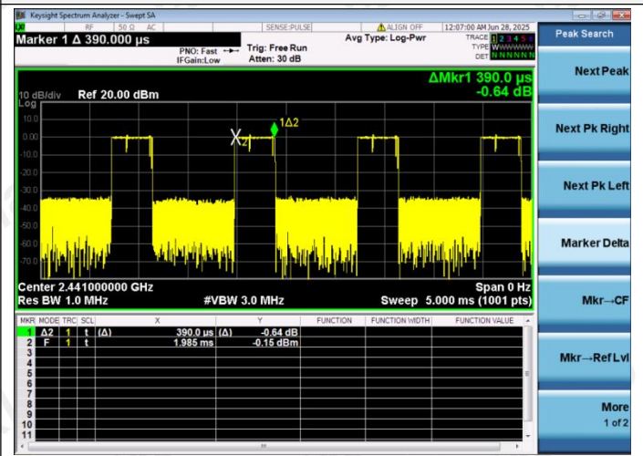
2-DH1 burst time
