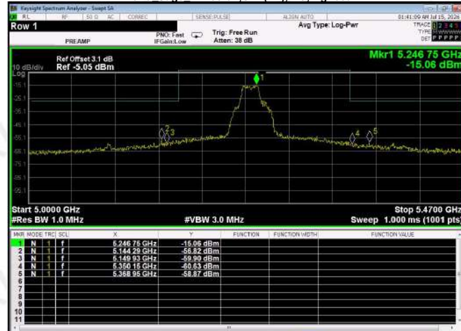
Band edge Emission,UNII(B1),11a,Highest
