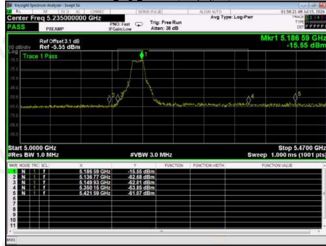
Band edge Emission,UNII(B1),11a,Lowest
