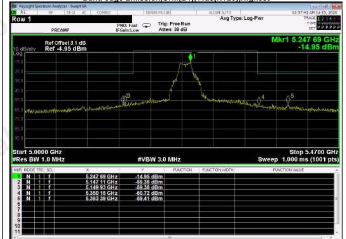
Band edge Emission,UNII(B1),11ac(HT20),Highest
