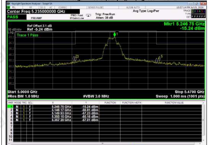
Band edge Emission,UNII(B1),11n,Highest
