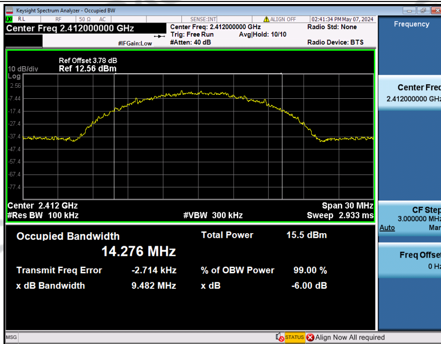
-6dB_Bandwidth_NVNT_ANT1_802_11b_2412
