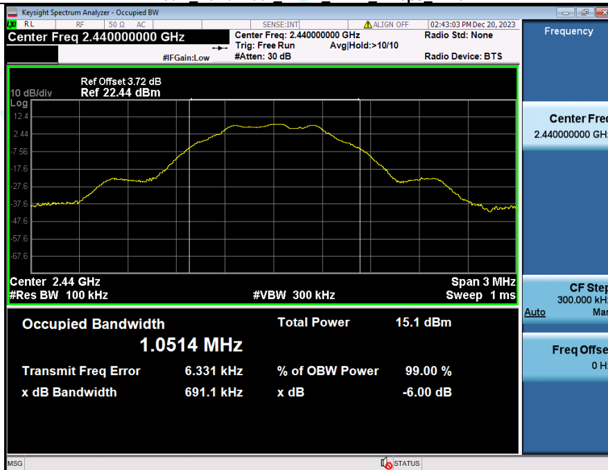
-6dB Bandwidth_NVNT_ANT1_1Mbps_2440
