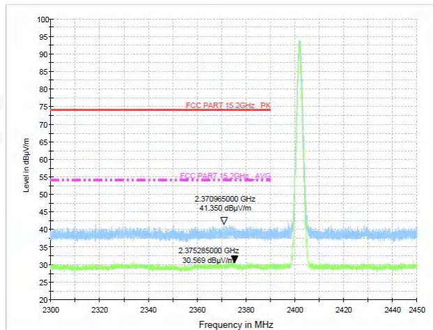
Test Mode: GFSK(2Mbps)-Low
