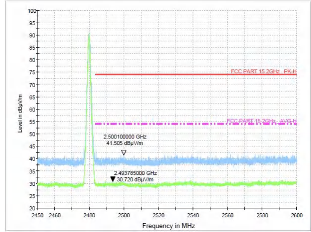
Test Mode: GFSK(1Mbps)-High
