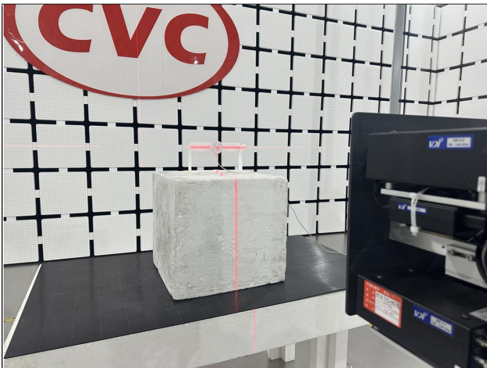
RADIATED EMISSION TEST (Above 40GHz-2)
