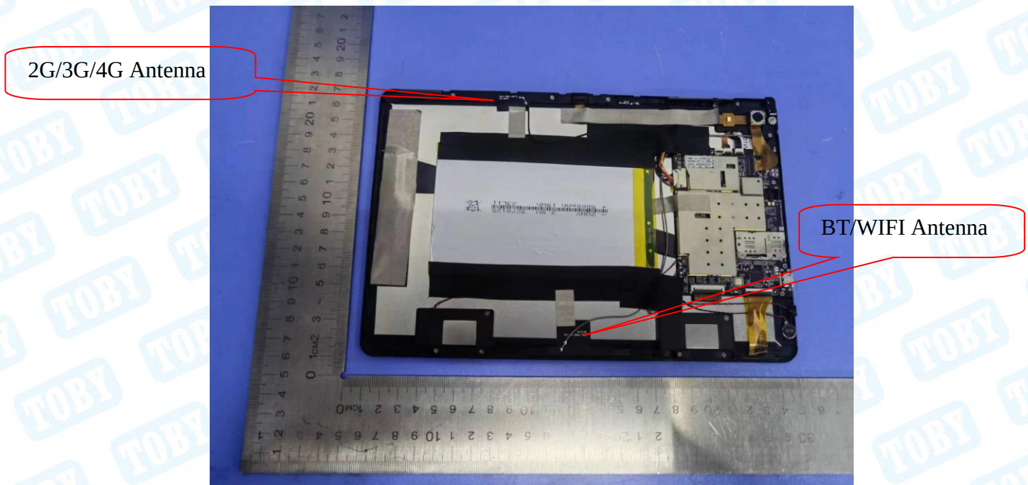
Photo 8 Internal of EUT
