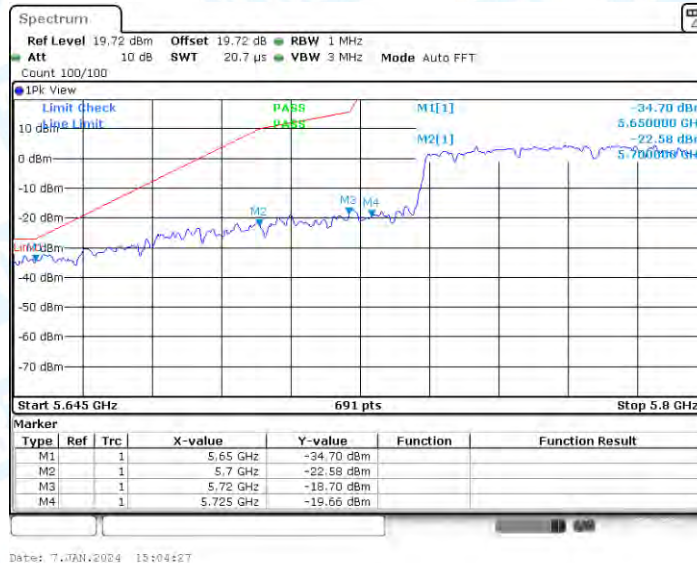
11AC80SISO_Ant1_High_5775_Peak
