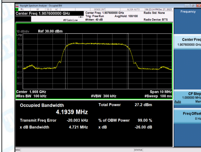
Band2-9400-4-PASS
