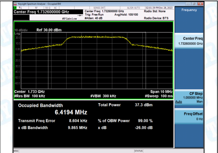
Band4-1312-3-PASS
