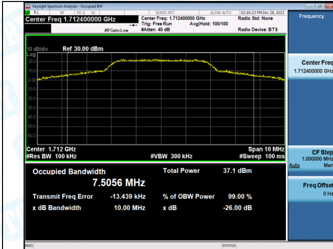
Band4-1513-2-PASS
