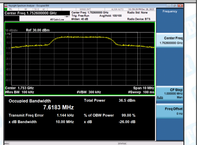
Band4-1413-2-PASS
