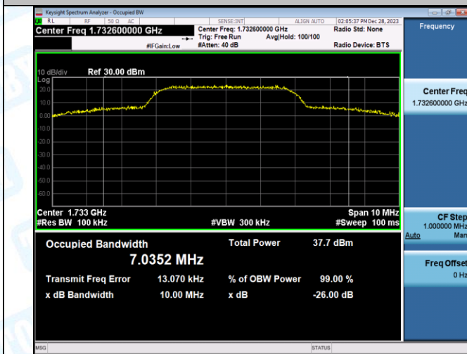
Band4-1312-4-PASS
