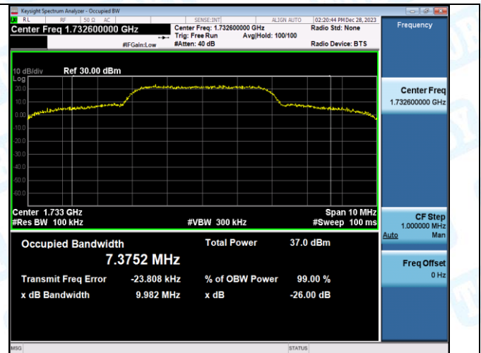
Band4-1312-5-PASS
