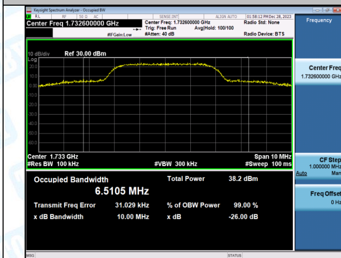
Band4-1312-2-PASS
