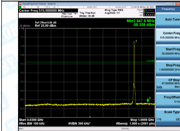
Band5-4233-30~1000MHz-PASS
