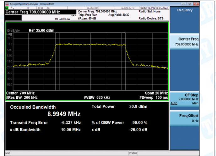
Band17-10MHz-16QAM-23790-50RB#0-PASS
