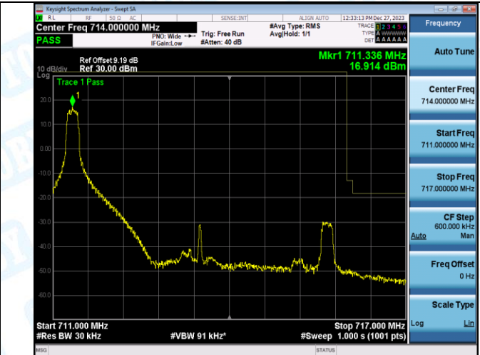
Band17_10MHz_QPSK_23780_1RB#0
