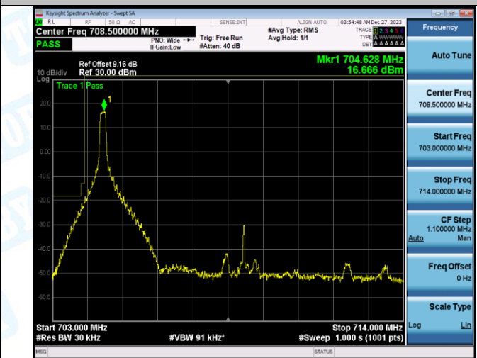
Band17_10MHz_QPSK_23780_1RB#49
