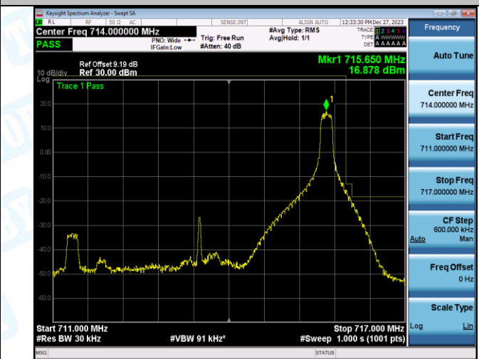
Band17_5MHz_16QAM_23825_25RB#0
