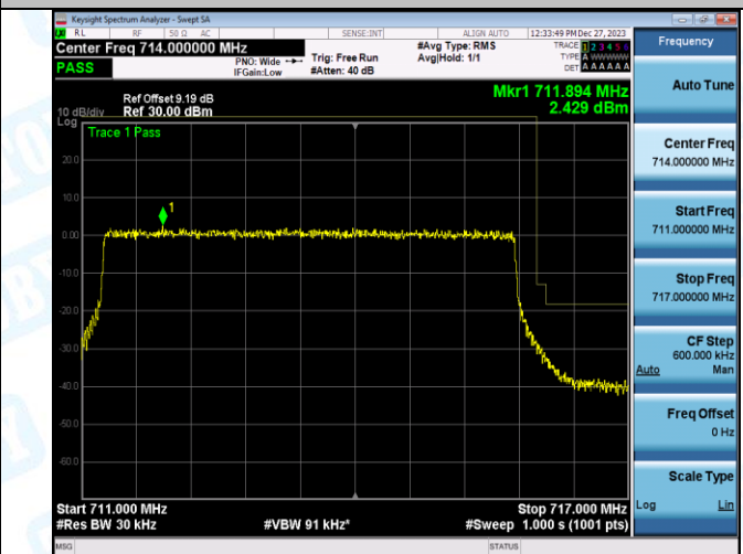
Band17_10MHz_16QAM_23800_1RB#0
