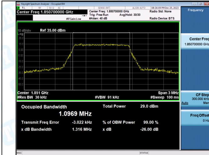
Band2-1.4MHz-16QAM-18900-6RB#0-PASS
