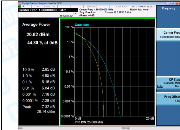
Band2-10MHz-QPSK-19150-1RB#0-PASS
