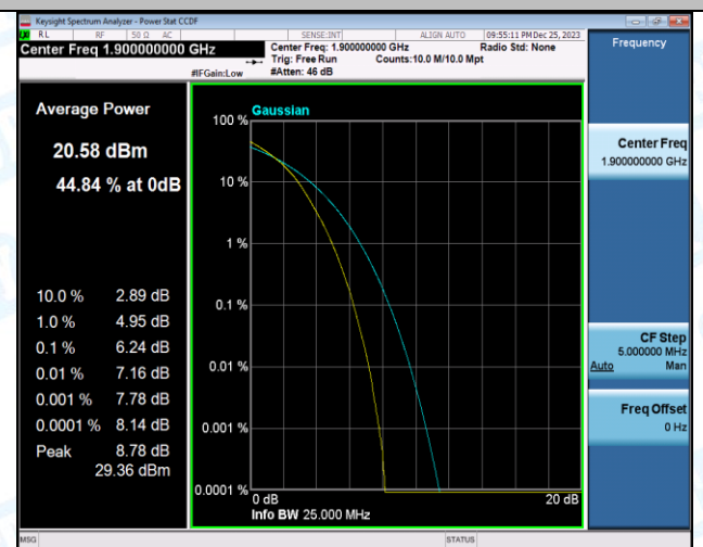
Band2-20MHz-16QAM-19100-100RB#0-PASS
