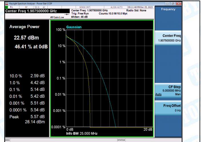
Band2-10MHz-16QAM-19150-1RB#0-PASS
