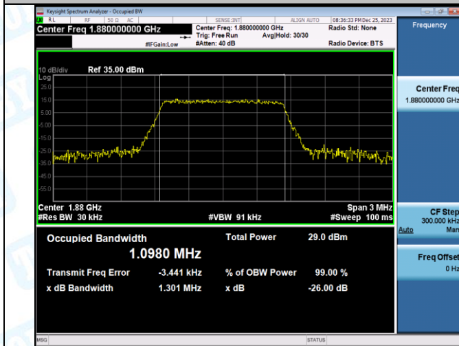
Band2-1.4MHz-16QAM-19193-6RB#0-PASS
