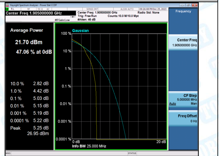
Band2-10MHz-16QAM-19150-50RB#0-PASS
