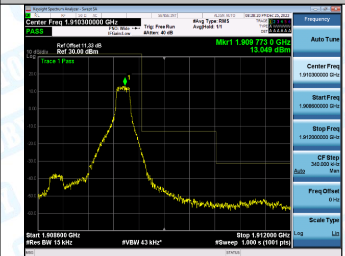
Band2_1.4MHz_QPSK_19193_6RB#0
