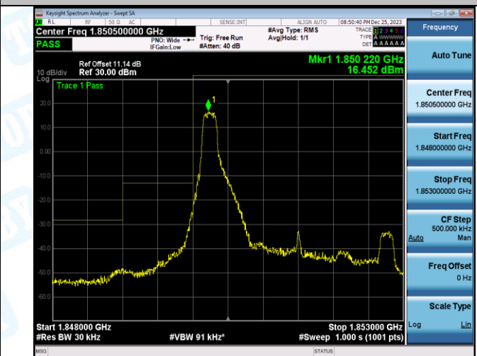
Band2_3MHz_QPSK_18615_1RB#14
