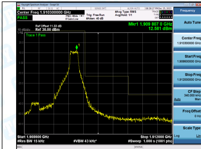
Band2_1.4MHz_16QAM_19193_6RB#0
