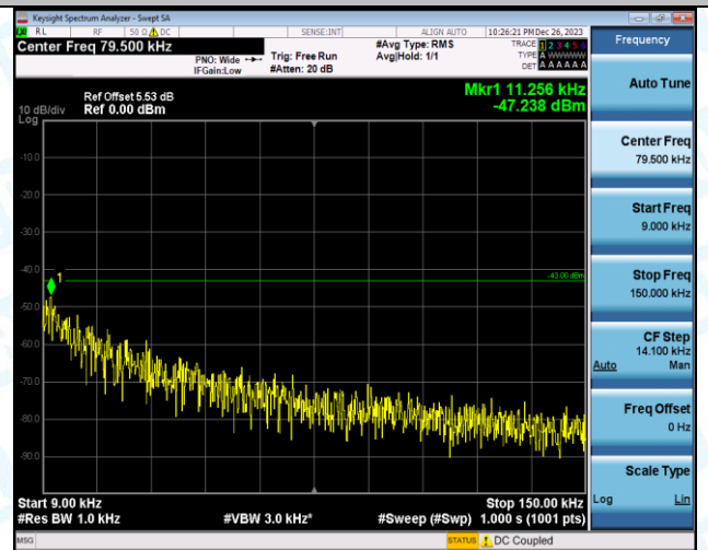
Band2_1.4MHz_16QAM_18900_1RB#0_0.009~0.15_0.009~0.15
