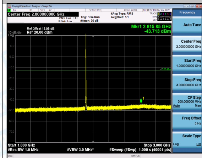
Band2_5MHz_QPSK_18625_1RB#0_0.009~0.15_0.009~0.15
