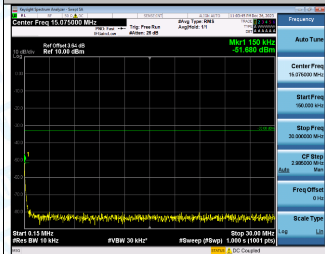
Band2_5MHz_16QAM_19175_1RB#0_1000~3000_1000~3000
